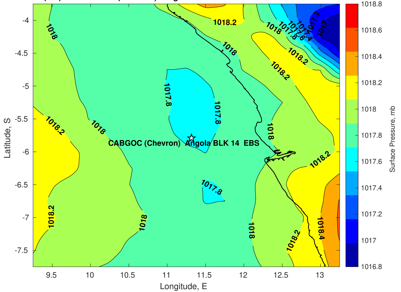
Surface Pressure (mb) for CABGOC (Chevron) Angola BLK 14 EBS at 15-Jul-2025 00:00:00
