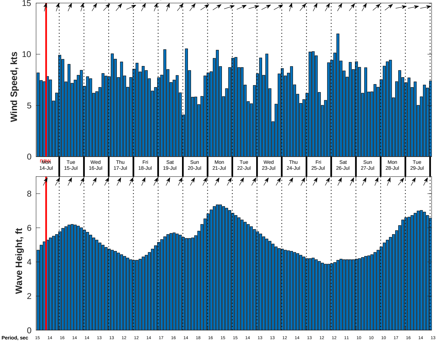
Wind & Wave Forecast for CABGOC (Chevron) Angola BLK 14 EBS from 13-Jul-2025 02:00:00 to 29-Jul-2025 02:00:00
