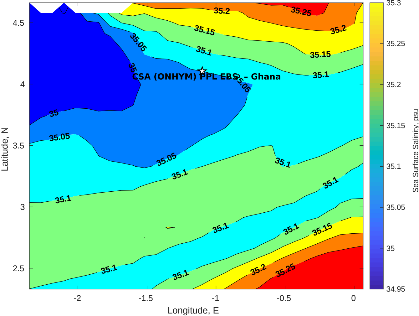
Surface Salinity for CSA (ONHYM) PPL EBS - Ghana at 12-Jul-2025 00:00:00
