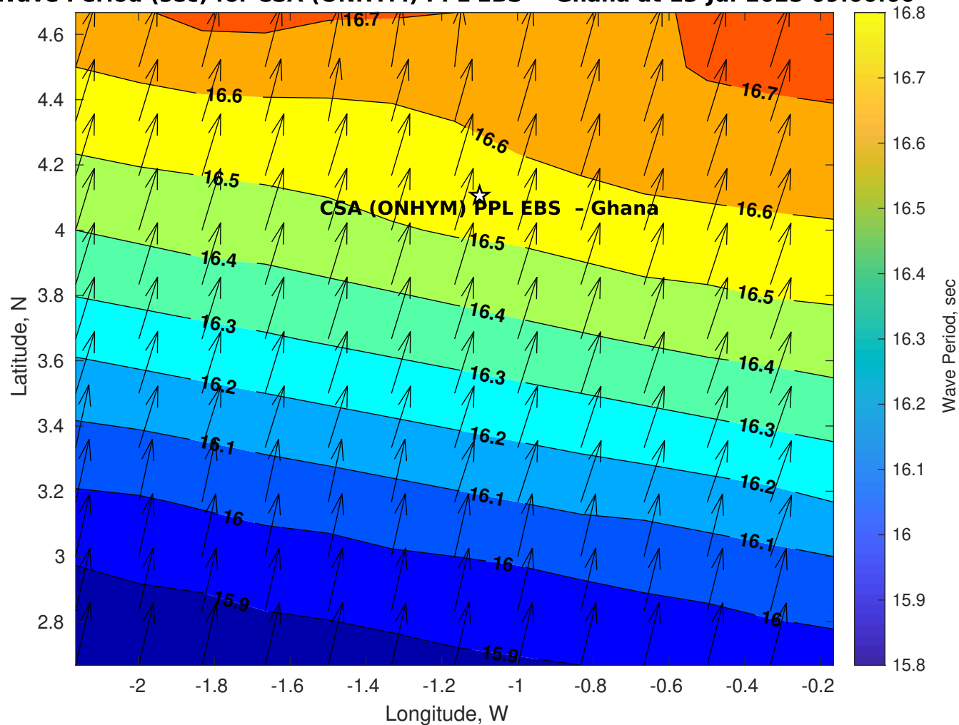
Wave Period (sec) for CSA (ONHYM) PPL EBS - Ghana at 13-Jul-2025 09:00:00
