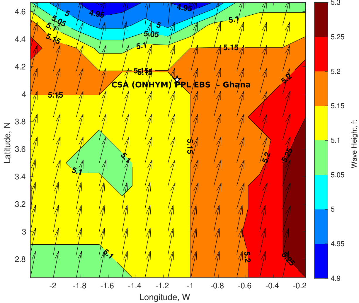
Wave Height (ft) for CSA (ONHYM) PPL EBS - Ghana at 13-Jul-2025 09:00:00
