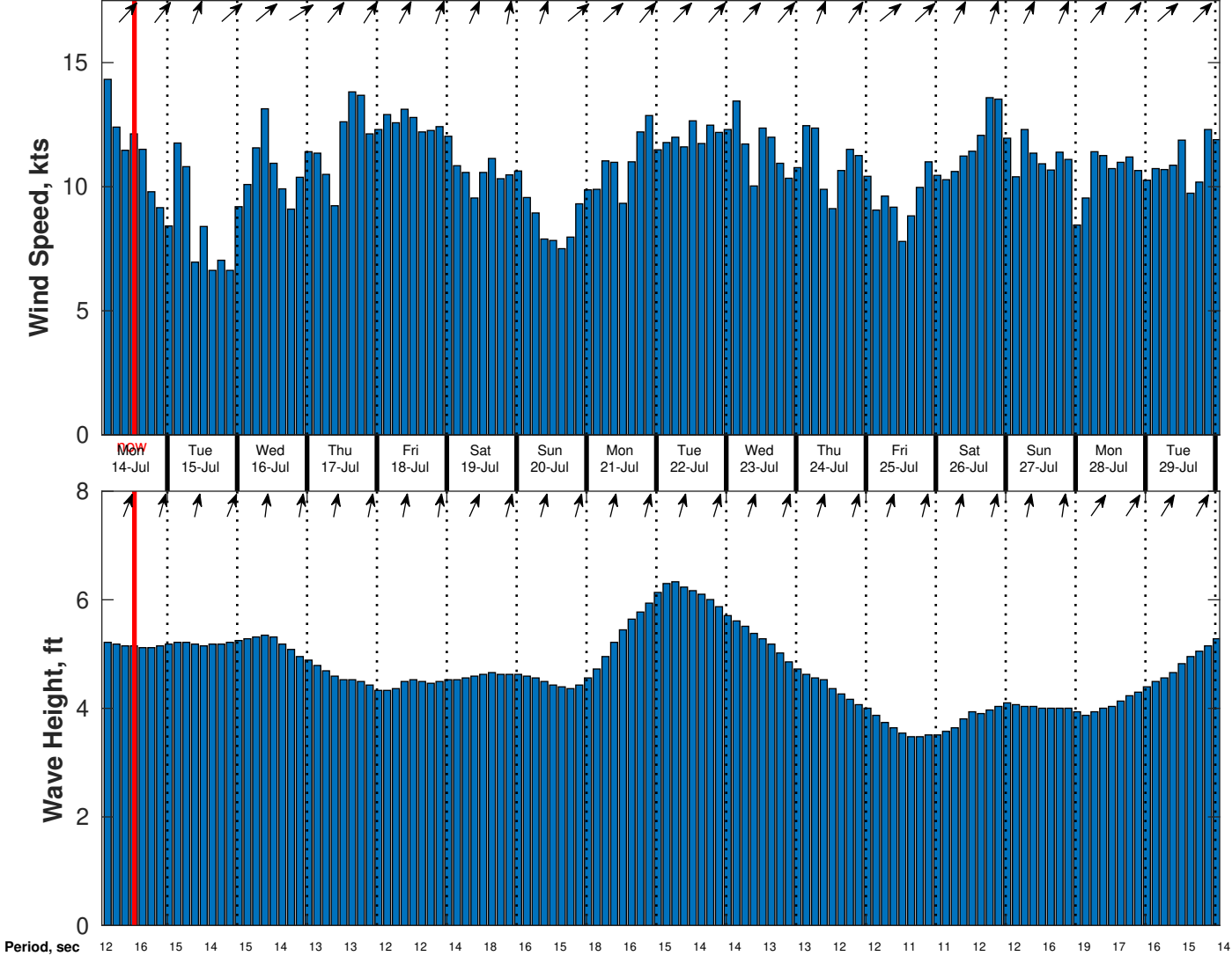
Wind & Wave Forecast for CSA (ONHYM) PPL EBS - Ghana from 13-Jul-2025 02:00:00 to 29-Jul-2025 02:00:00
