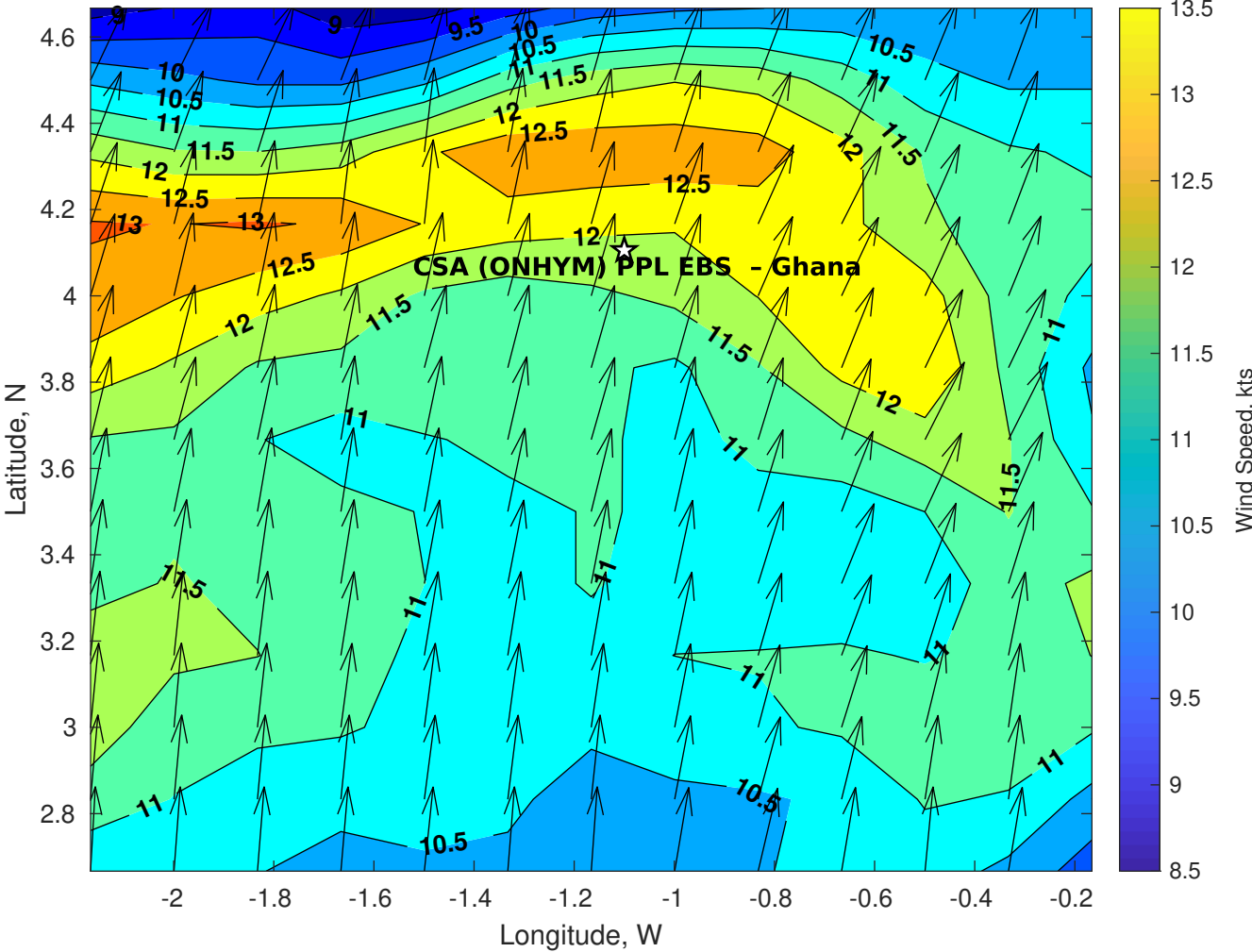
Winds (kts) for CSA (ONHYM) PPL EBS - Ghana at 13-Jul-2025 09:00:00
