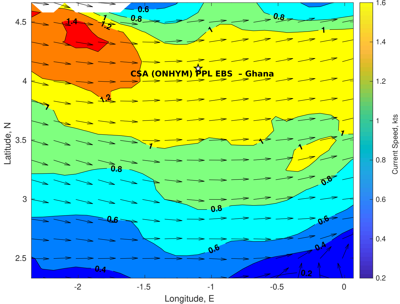
Surface Currents for CSA (ONHYM) PPL EBS - Ghana at 12-Jul-2025 00:00:00
