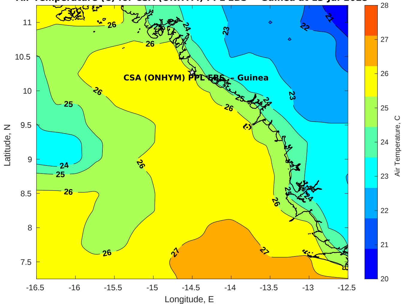
Air Temperature (C) for CSA (ONHYM) PPL EBS - Guinea at 13-Jul-2025
