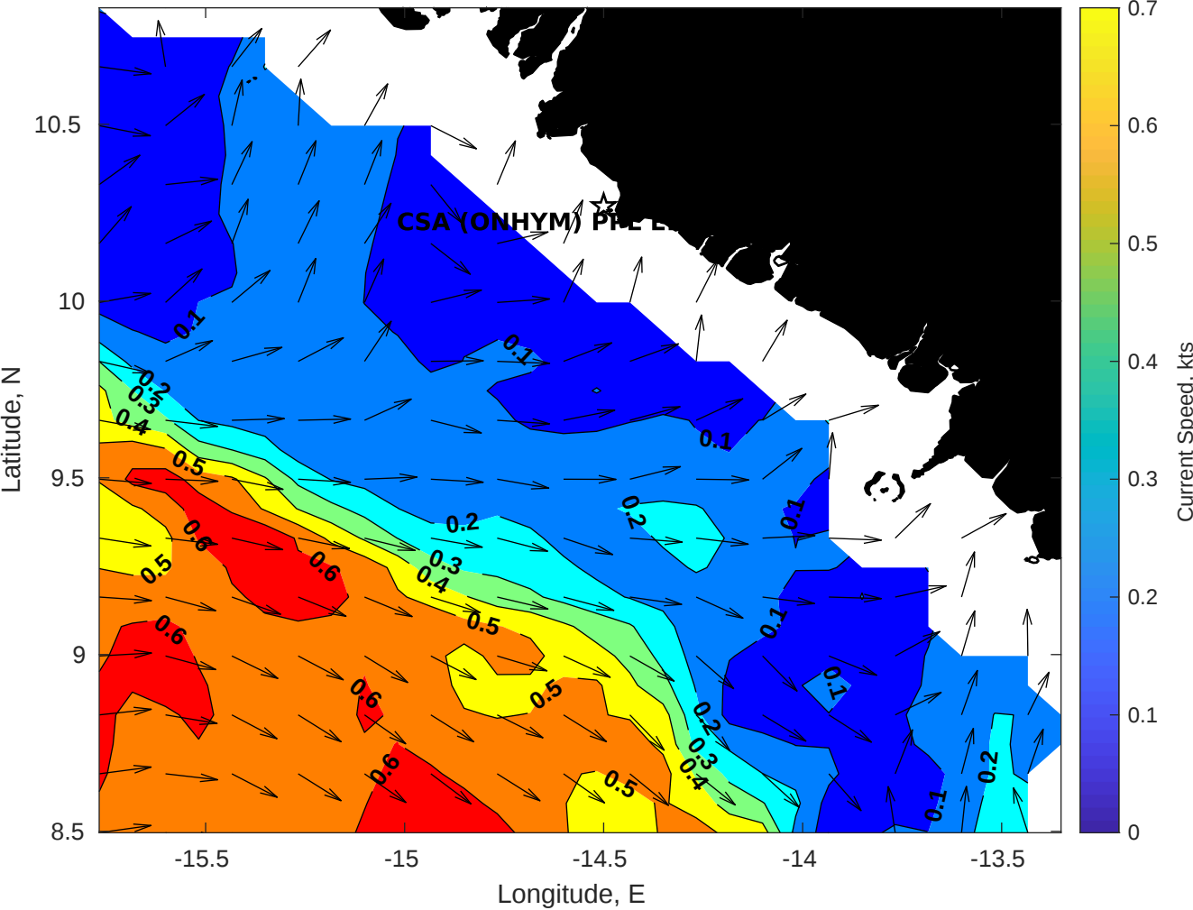
Surface Currents for CSA (ONHYM) PPL EBS - Guinea at 12-Jul-2025 00:00:00
