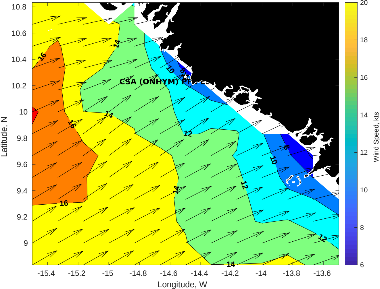
Winds (kts) for CSA (ONHYM) PPL EBS - Guinea at 13-Jul-2025 09:00:00
