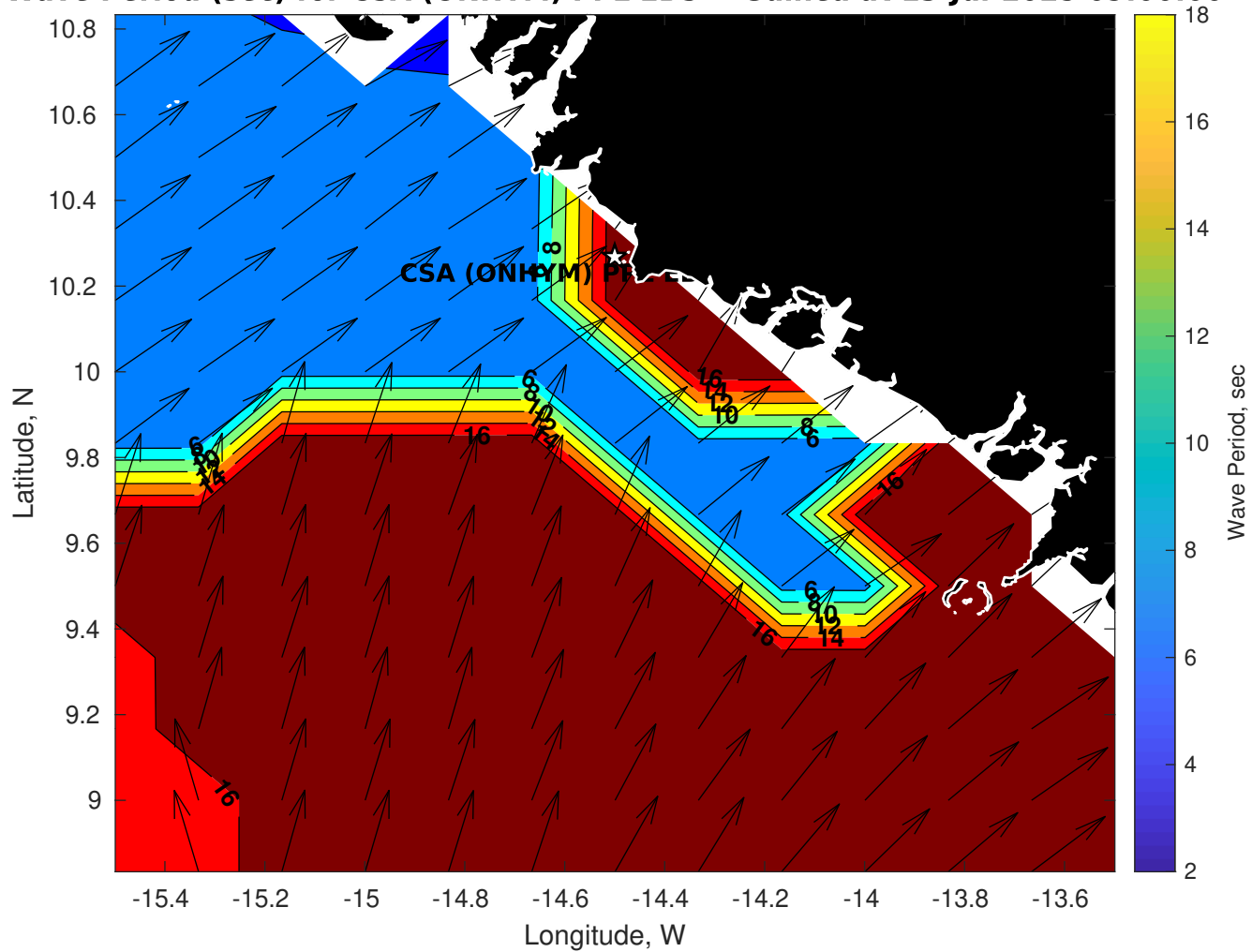
Wave Period (sec) for CSA (ONHYM) PPL EBS - Guinea at 13-Jul-2025 09:00:00
