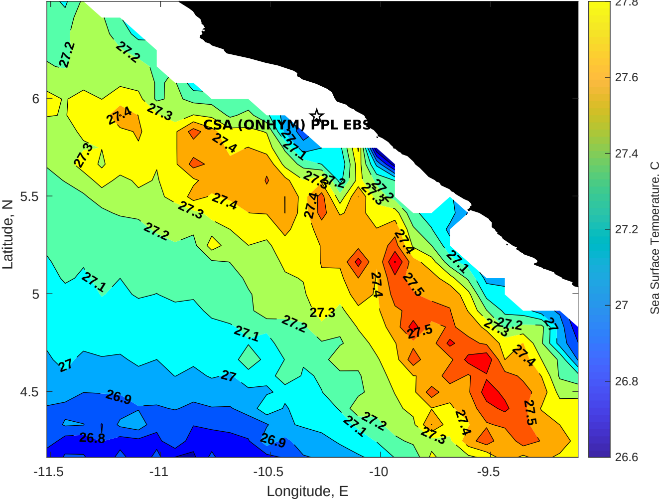
SST for CSA (ONHYM) PPL EBS - Liberia at 12-Jul-2025 00:00:00
