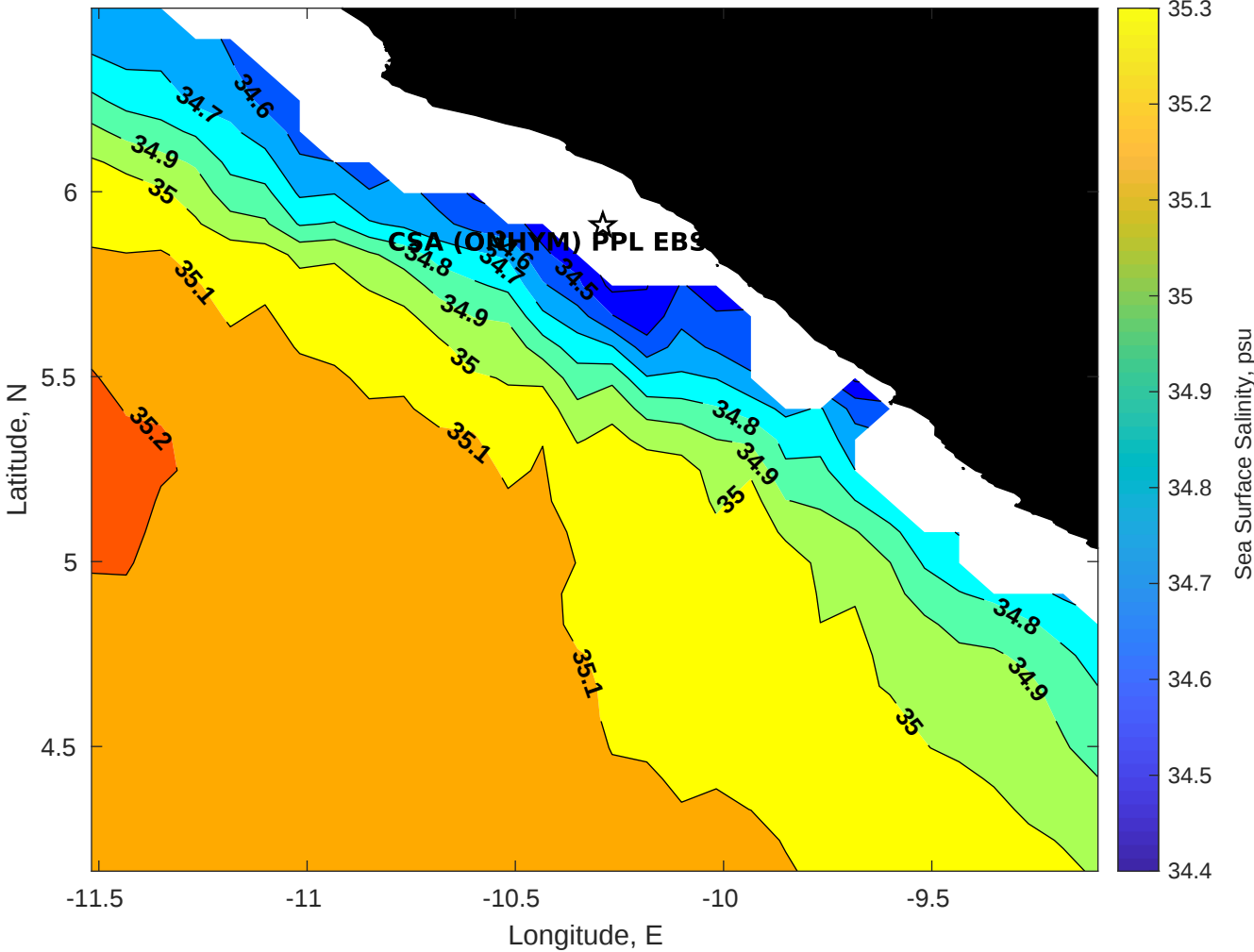
Surface Salinity for CSA (ONHYM) PPL EBS - Liberia at 12-Jul-2025 00:00:00
