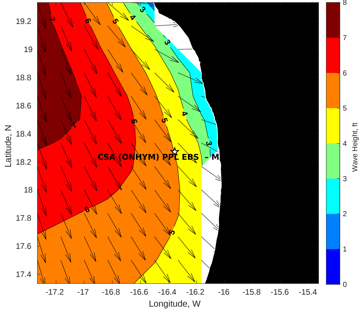
Wave Height (ft) for CSA (ONHYM) PPL EBS - Mauritania at 13-Jul-2025 09:00:00
