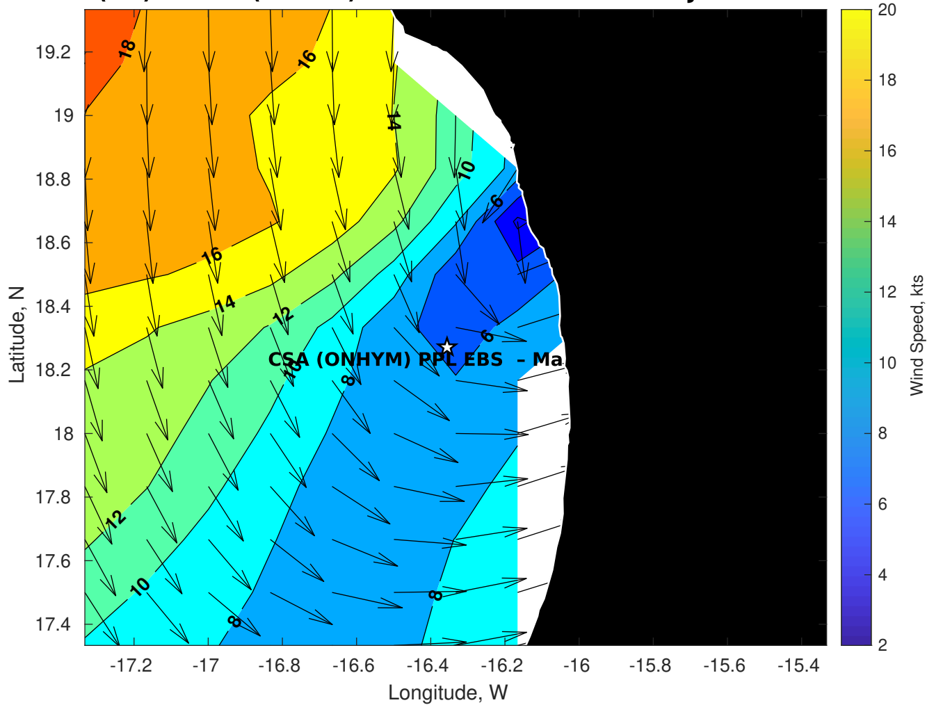
Winds (kts) for CSA (ONHYM) PPL EBS - Mauritania at 13-Jul-2025 09:00:00
