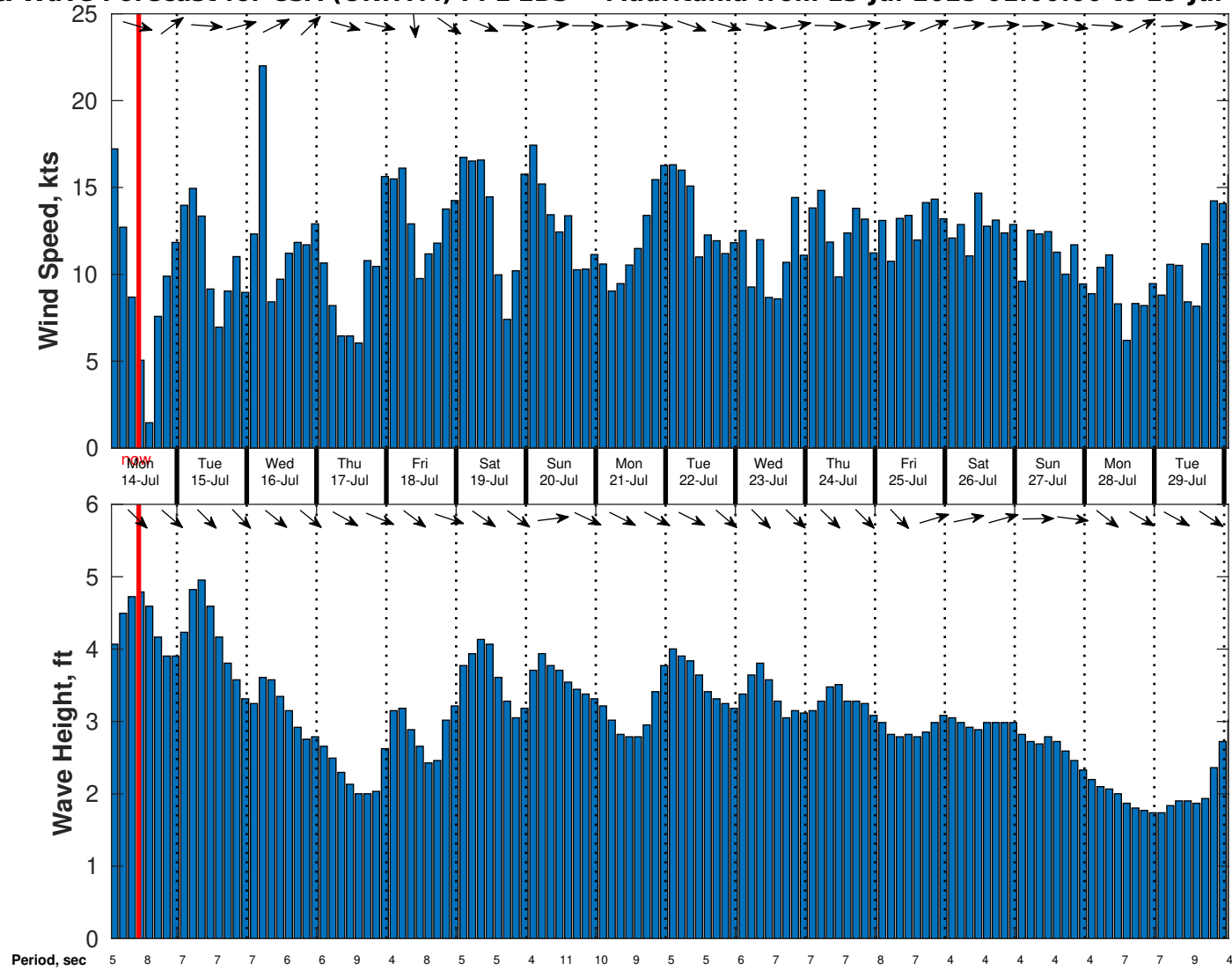
Wind & Wave Forecast for CSA (ONHYM) PPL EBS - Mauritania from 13-Jul-2025 01:00:00 to 29-Jul-2025 01:00:00
