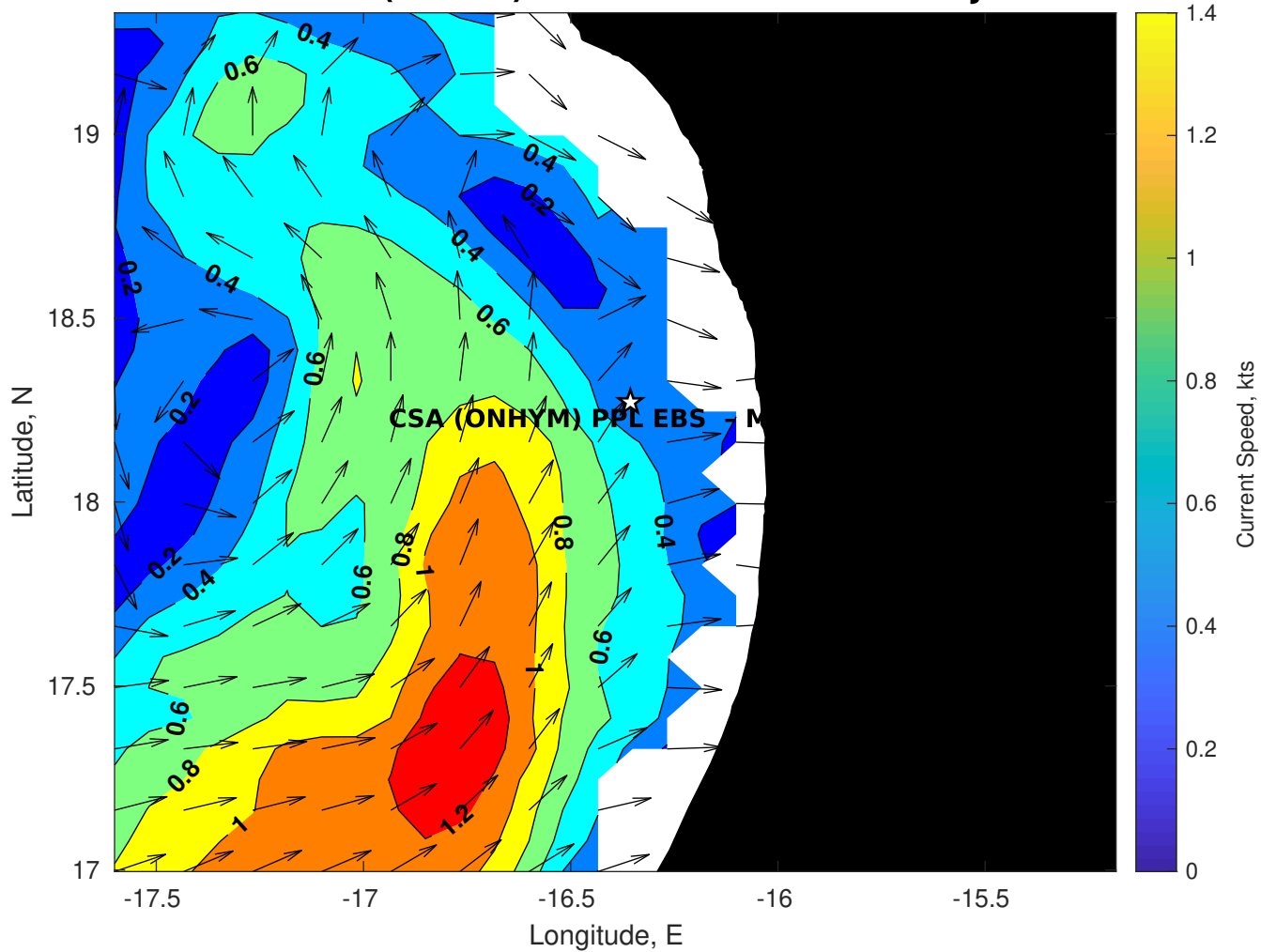
Surface Currents for CSA (ONHYM) PPL EBS - Mauritania at 12-Jul-2025 00:00:00
