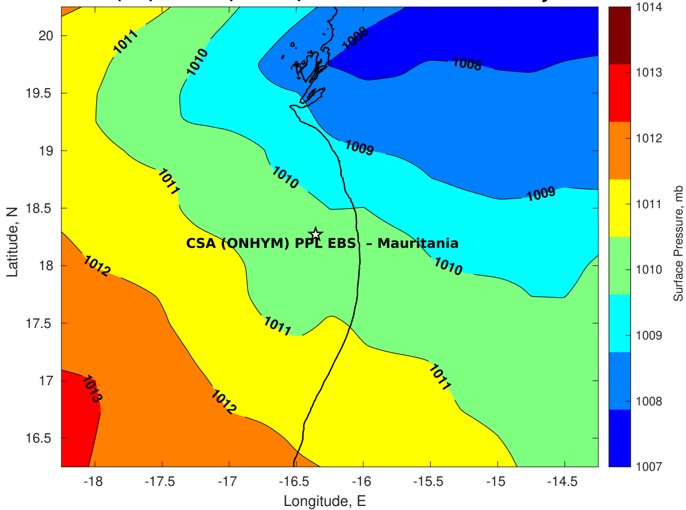
Surface Pressure (mb) for CSA (ONHYM) PPL EBS - Mauritania at 13-Jul-2025 00:00:00
