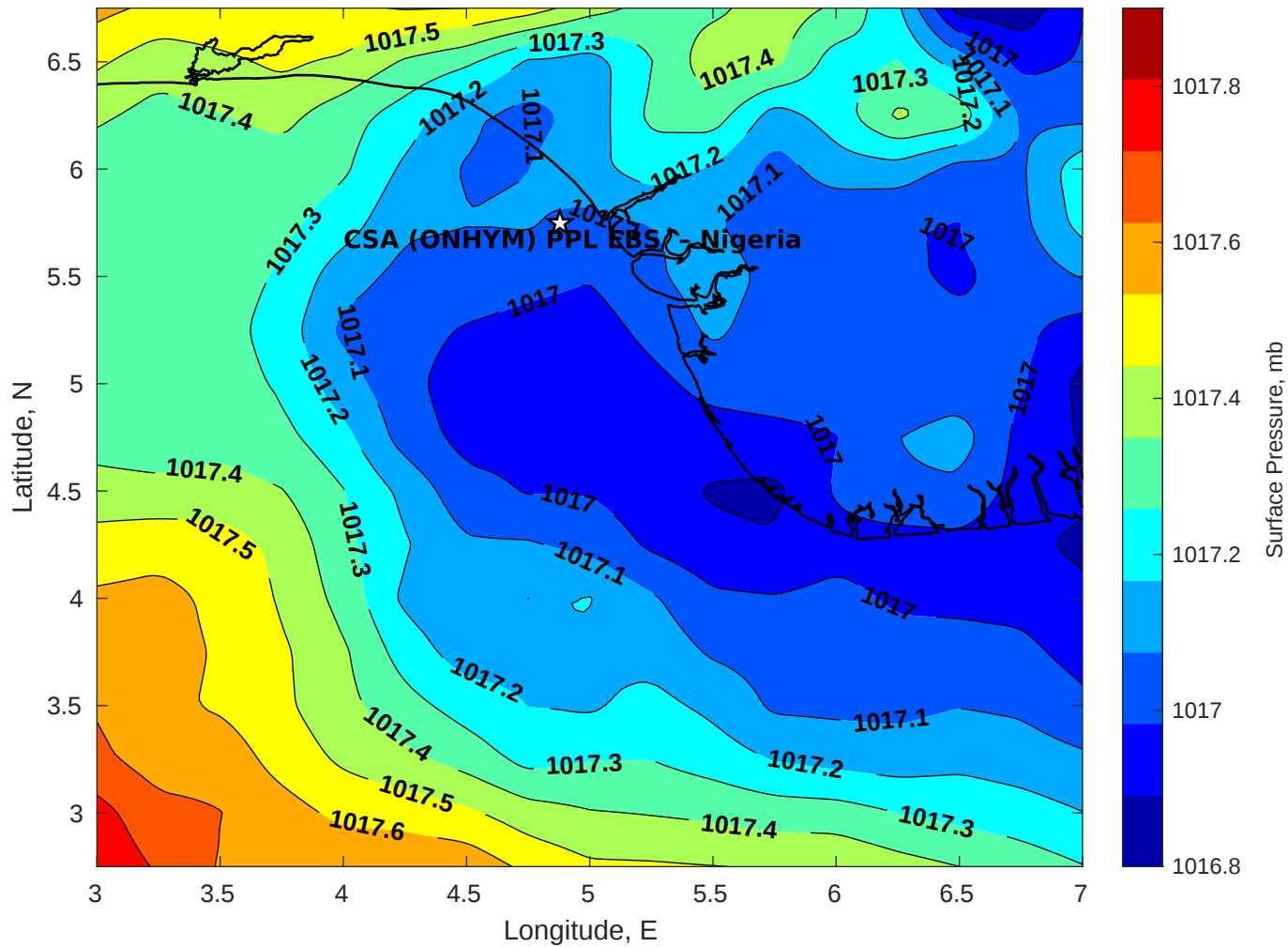
Surface Pressure (mb) for CSA (ONHYM) PPL EBS - Nigeria at 14-Jul-2025 00:00:00
