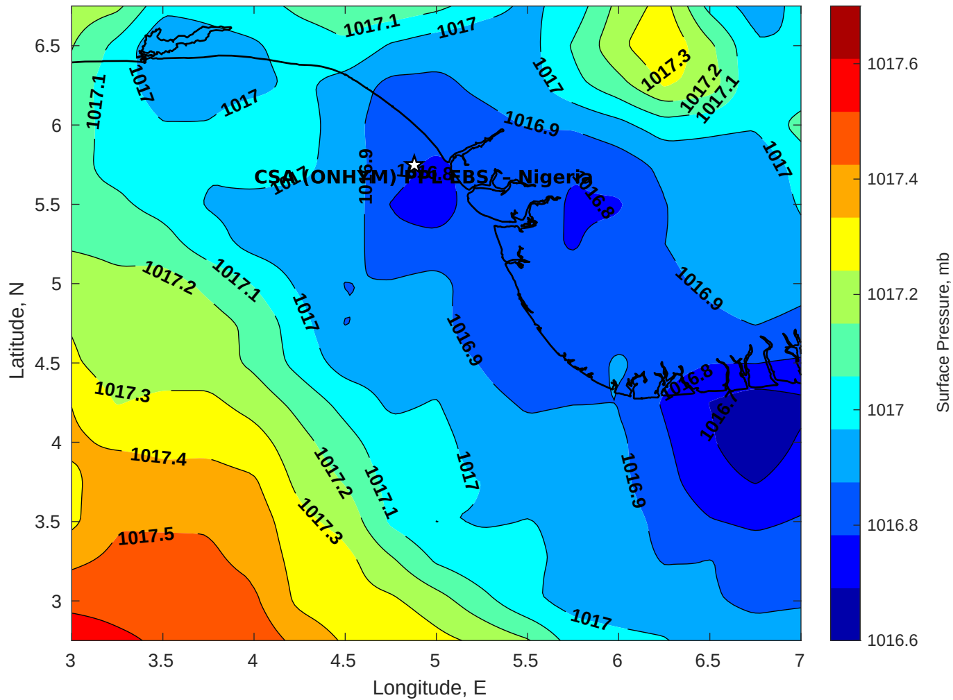
Surface Pressure (mb) for CSA (ONHYM) PPL EBS - Nigeria at 15-Jul-2025 00:00:00
