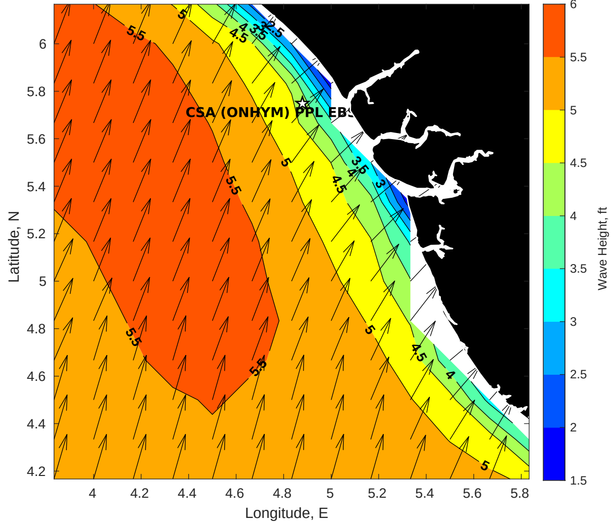
Wave Height (ft) for CSA (ONHYM) PPL EBS - Nigeria at 13-Jul-2025 09:00:00
