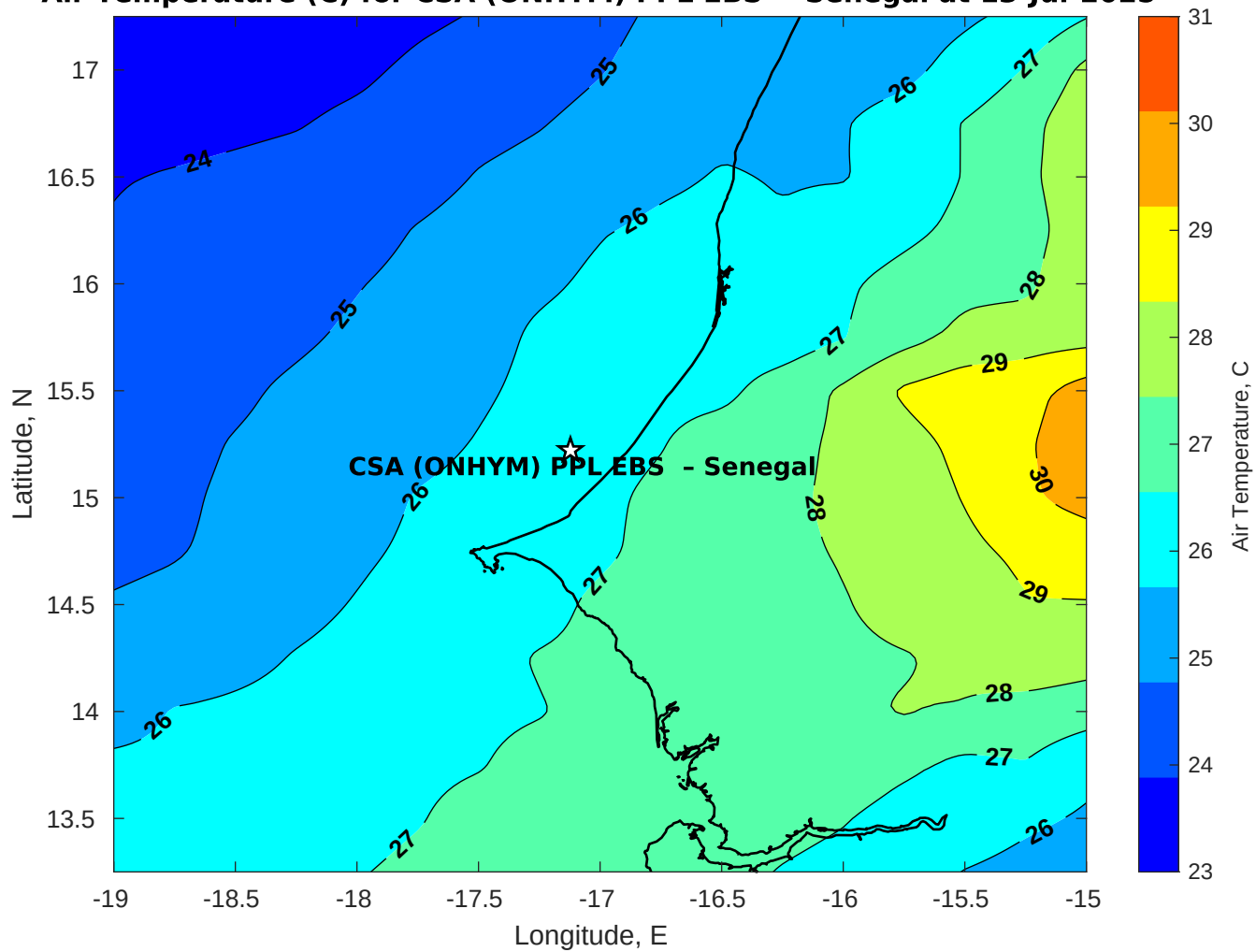
Air Temperature (C) for CSA (ONHYM) PPL EBS - Senegal at 13-Jul-2025
