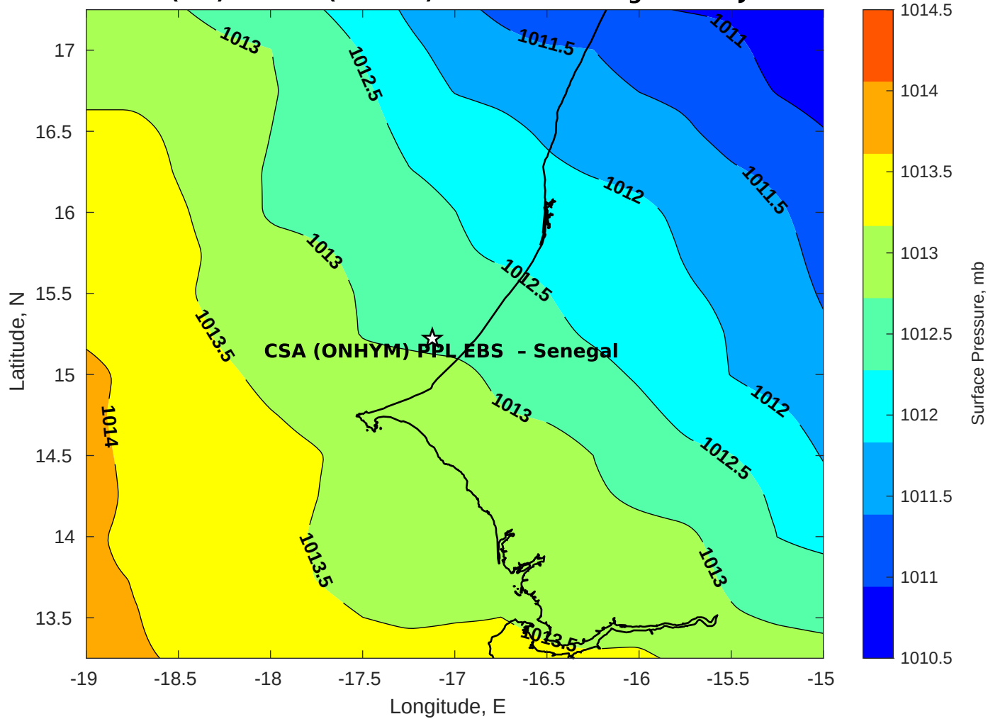
Surface Pressure (mb) for CSA (ONHYM) PPL EBS - Senegal at 13-Jul-2025 00:00:00
