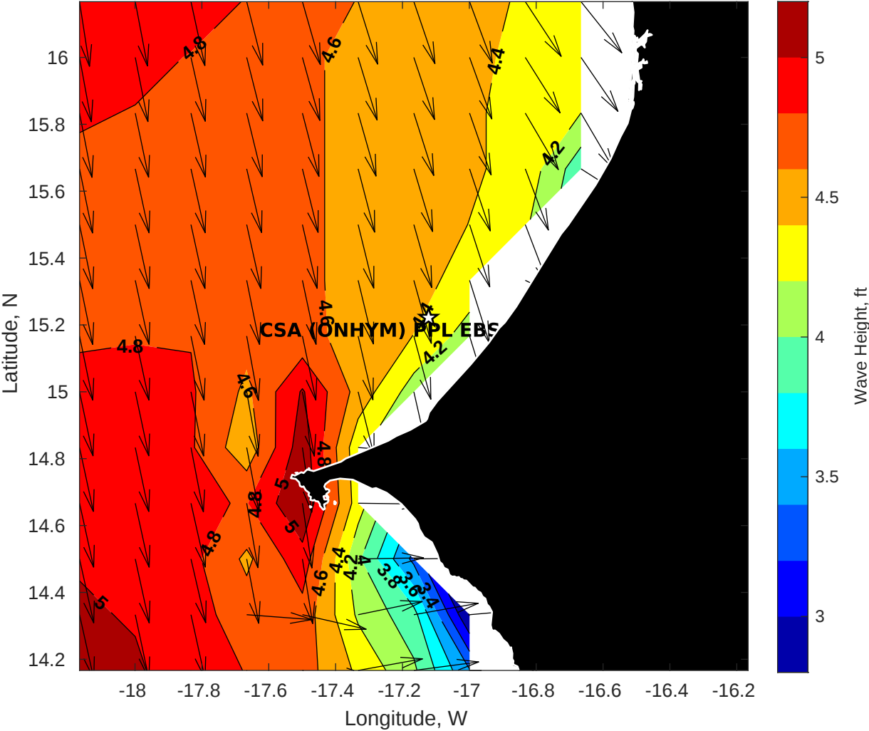
Wave Height (ft) for CSA (ONHYM) PPL EBS - Senegal at 13-Jul-2025 09:00:00
