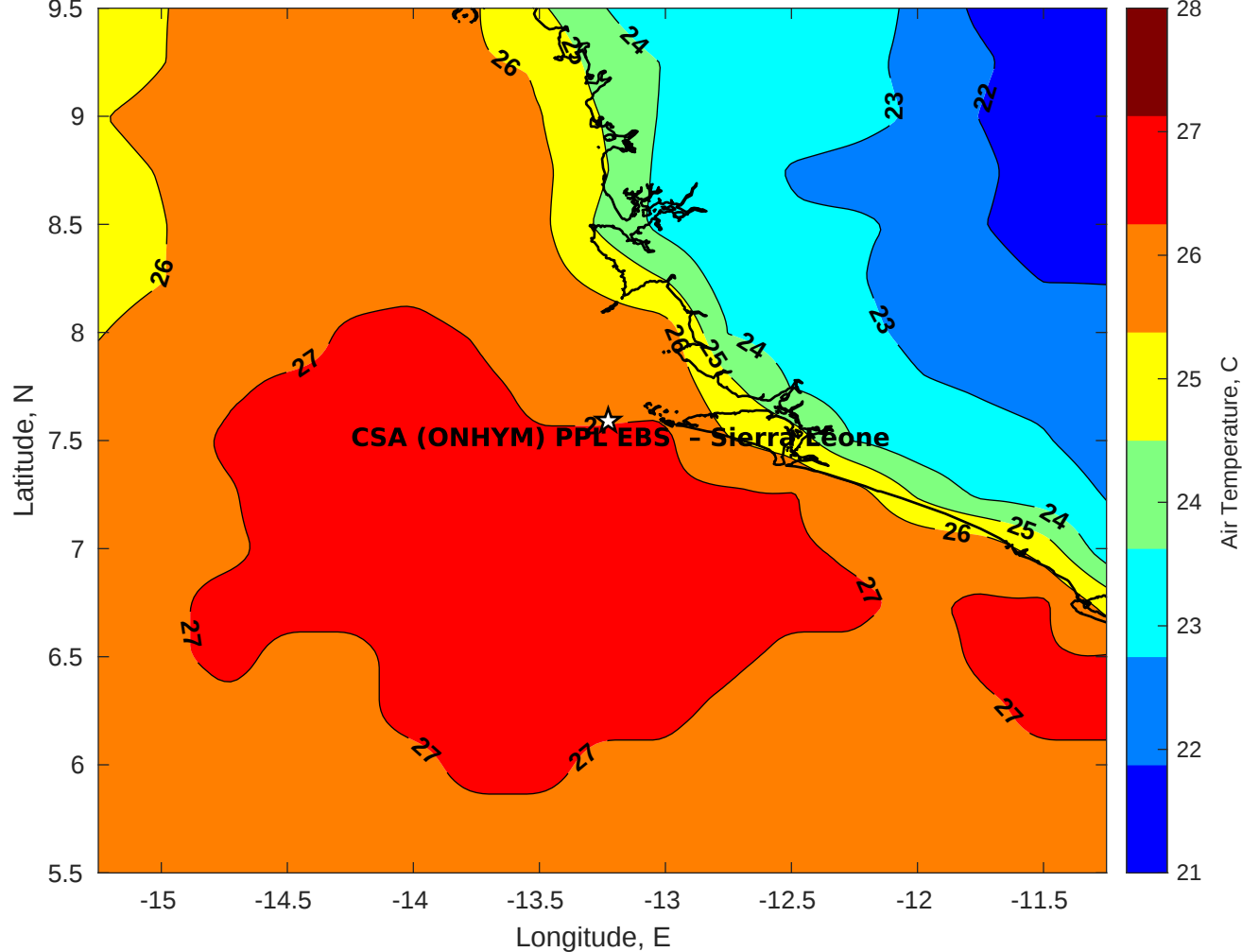
Air Temperature (C) for CSA (ONHYM) PPL EBS - Sierra Leone at 13-Jul-2025
