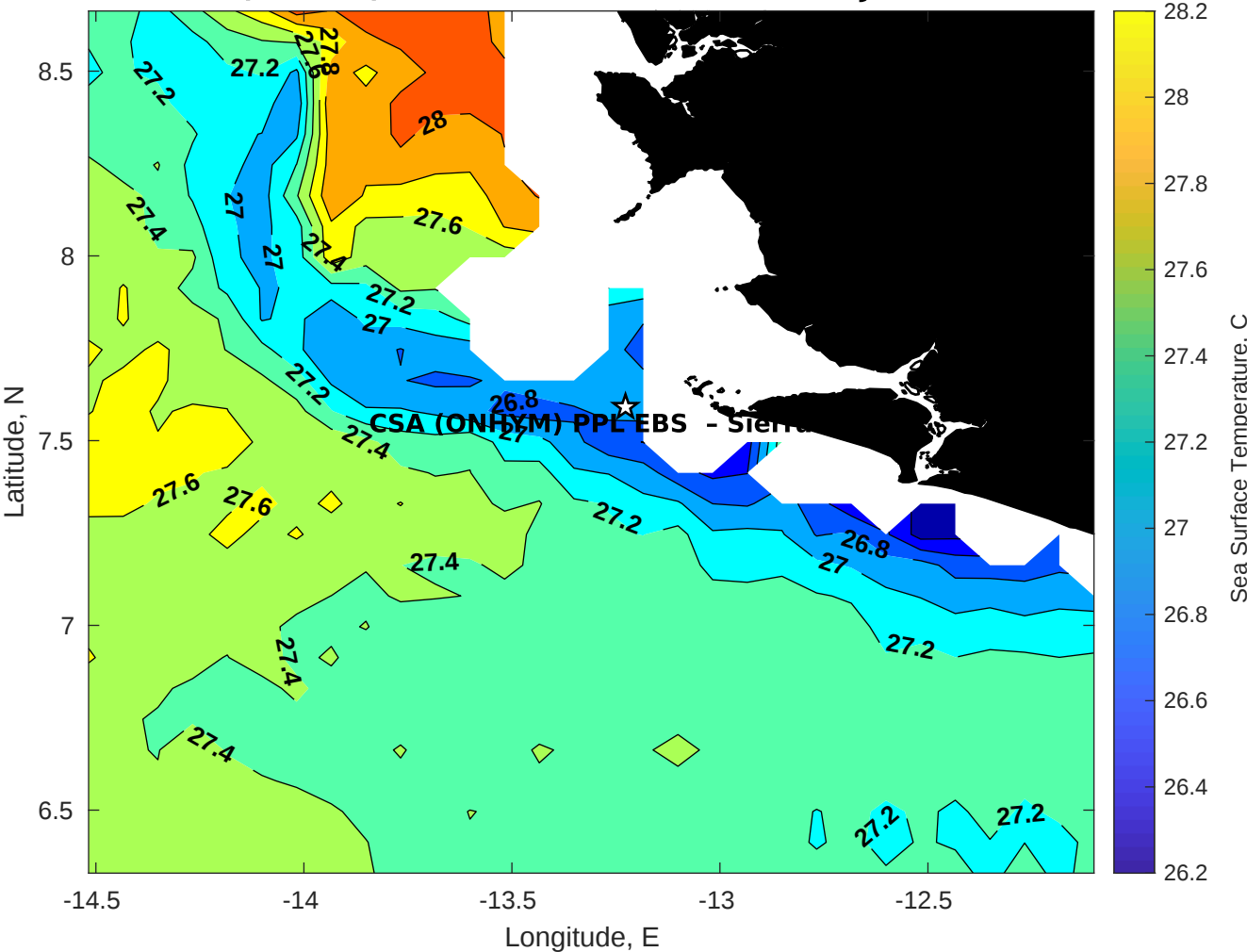
SST for CSA (ONHYM) PPL EBS - Sierra Leone at 12-Jul-2025 00:00:00
