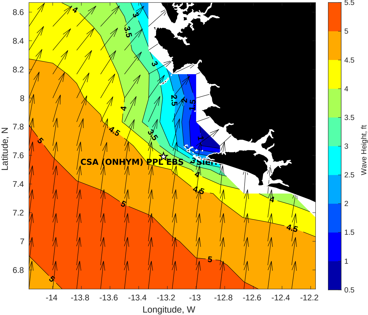
Wave Height (ft) for CSA (ONHYM) PPL EBS - Sierra Leone at 13-Jul-2025 09:00:00
