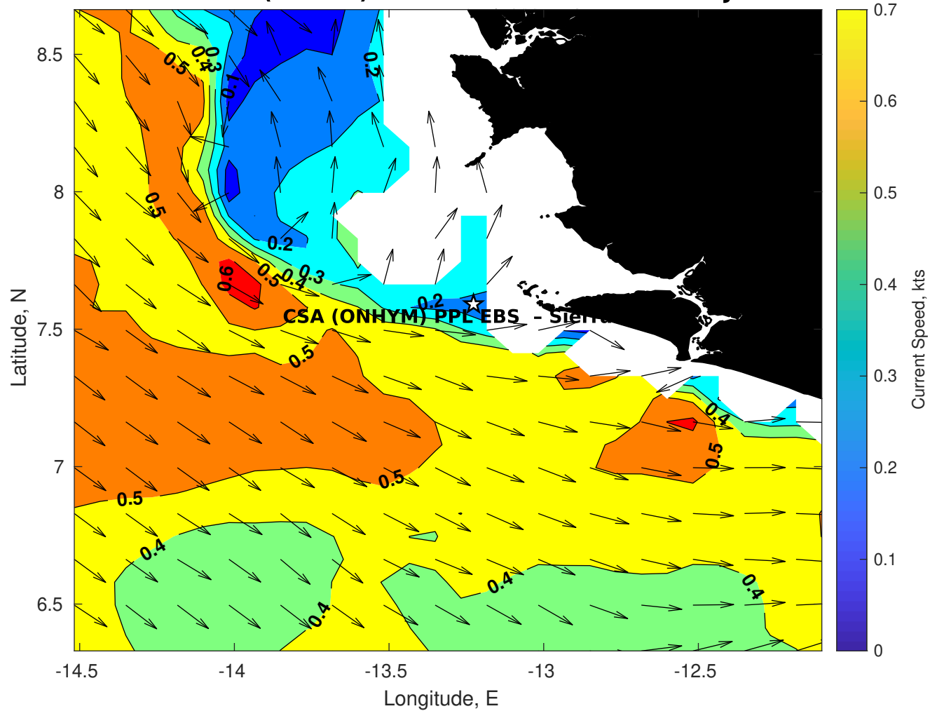
Surface Currents for CSA (ONHYM) PPL EBS - Sierra Leone at 12-Jul-2025 00:00:00
