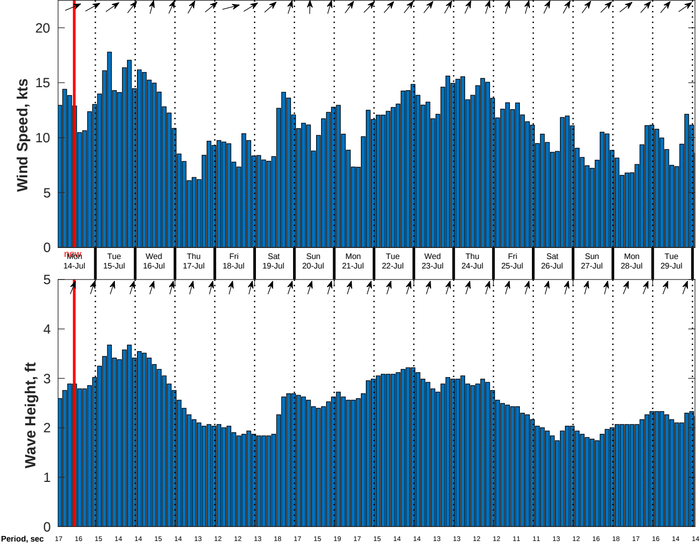
Wind & Wave Forecast for CSA (ONHYM) PPL EBS - Sierra Leone from 13-Jul-2025 01:00:00 to 29-Jul-2025 01:00:00
