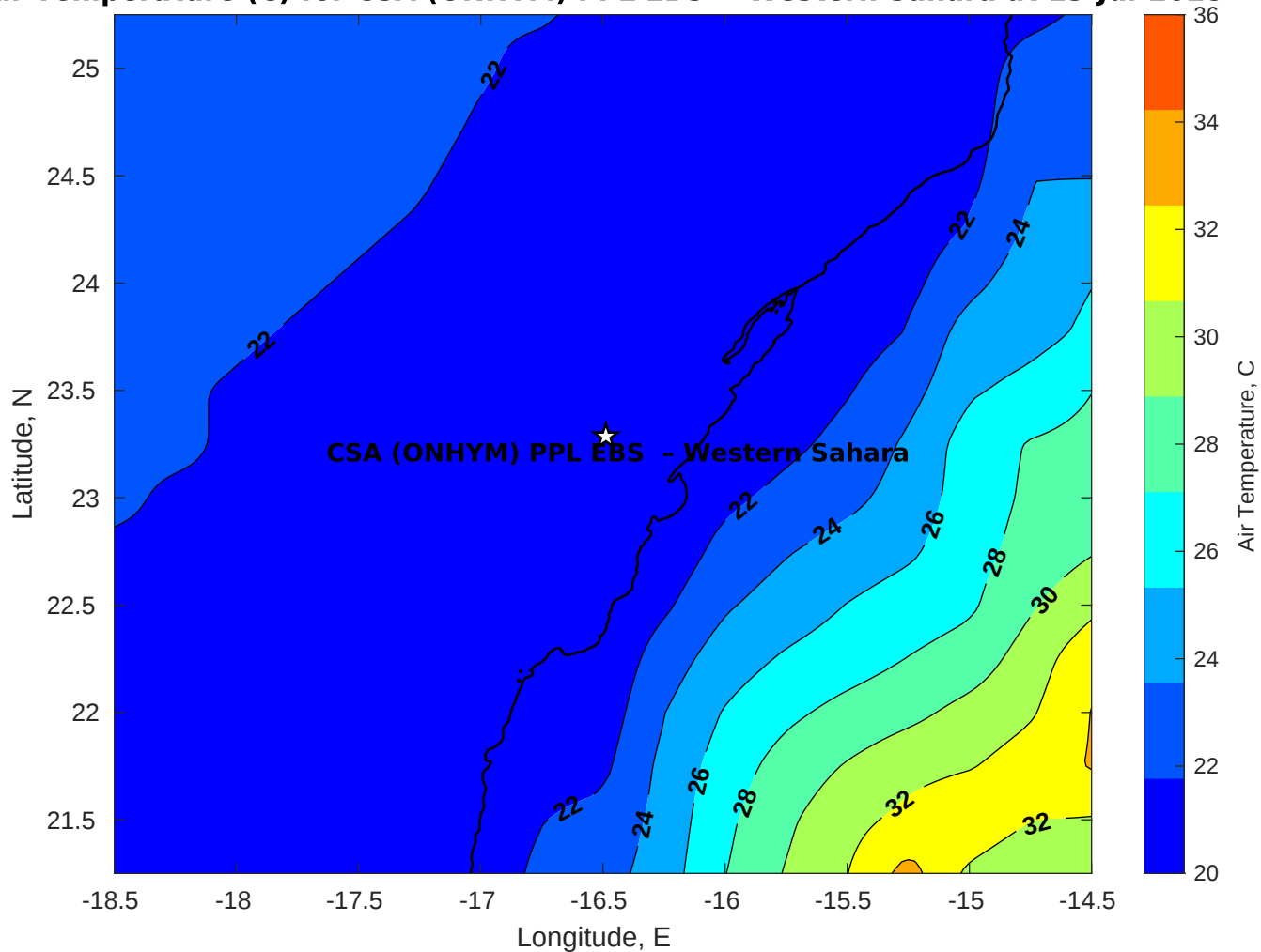
Air Temperature (C) for CSA (ONHYM) PPL EBS - Western Sahara at 13-Jul-2025
