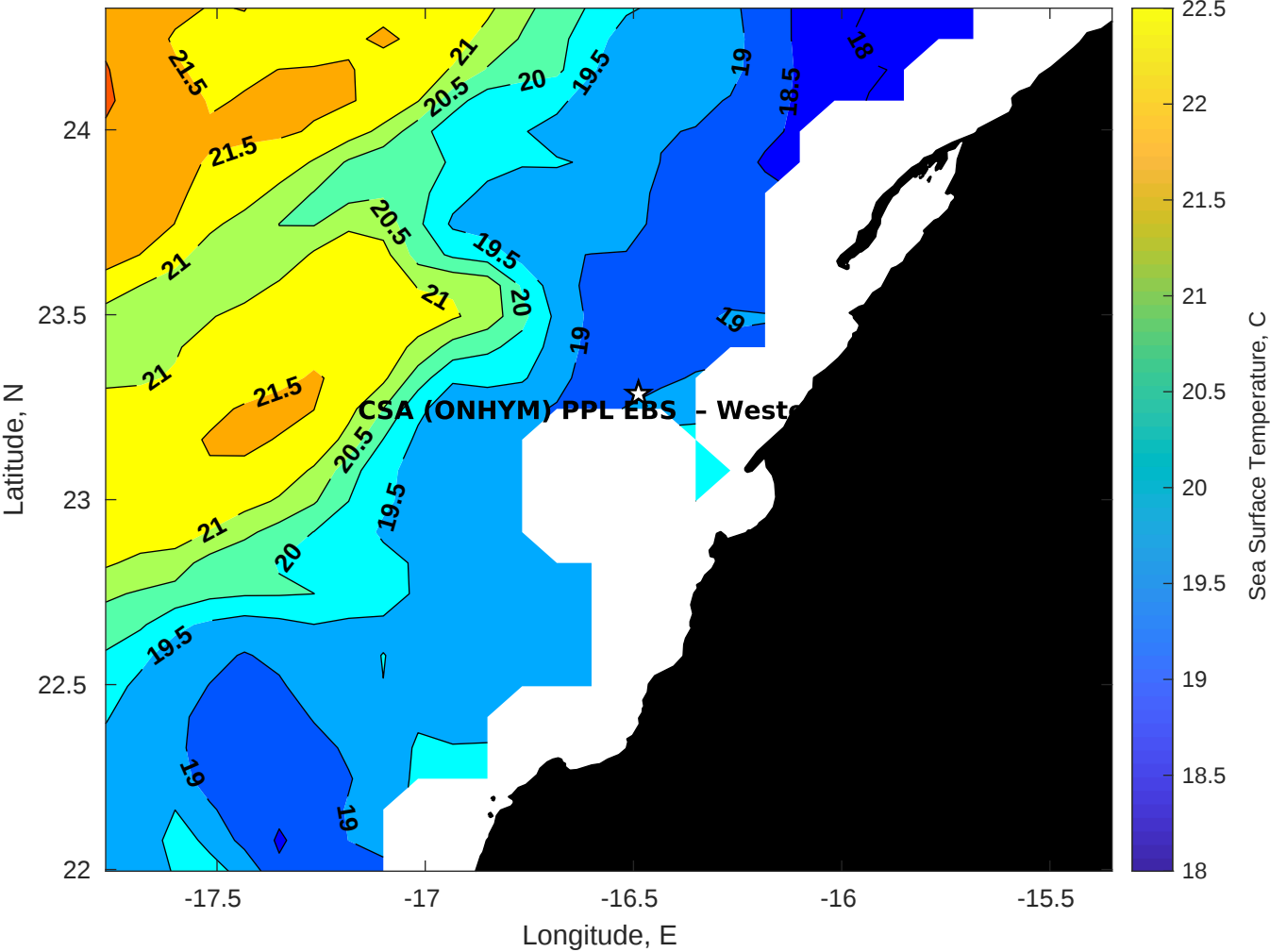
SST for CSA (ONHYM) PPL EBS - Western Sahara at 12-Jul-2025 00:00:00
