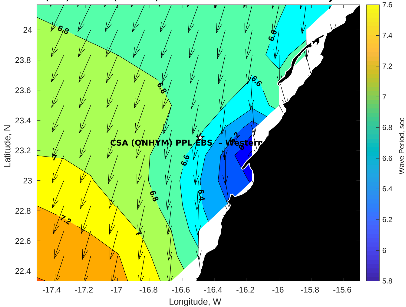
Wave Period (sec) for CSA (ONHYM) PPL EBS - Western Sahara at 13-Jul-2025 09:00:00
