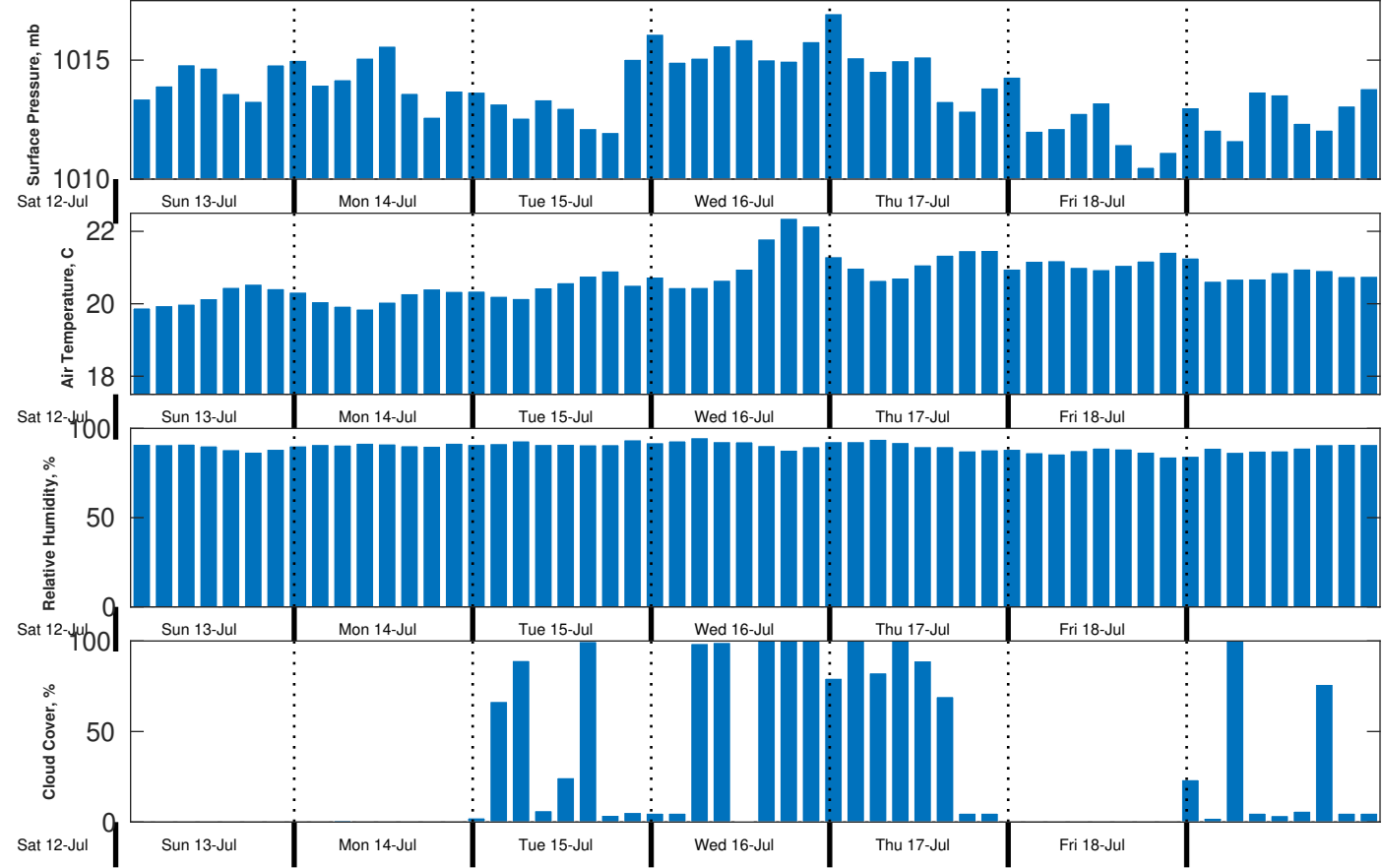
Met Forecast for CSA (ONHYM) PPL EBS - Western Sahara from 13-Jul-2025 00:00:00 to 20-Jul-2025 00:00:00
