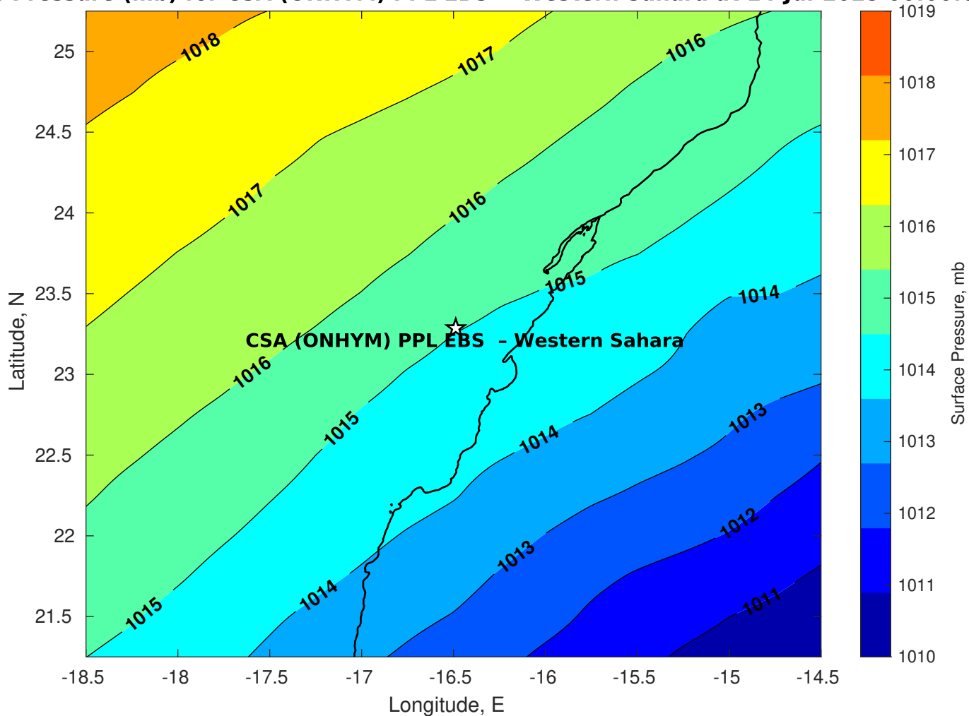
Surface Pressure (mb) for CSA (ONHYM) PPL EBS - Western Sahara at 14-Jul-2025 00:00:00
