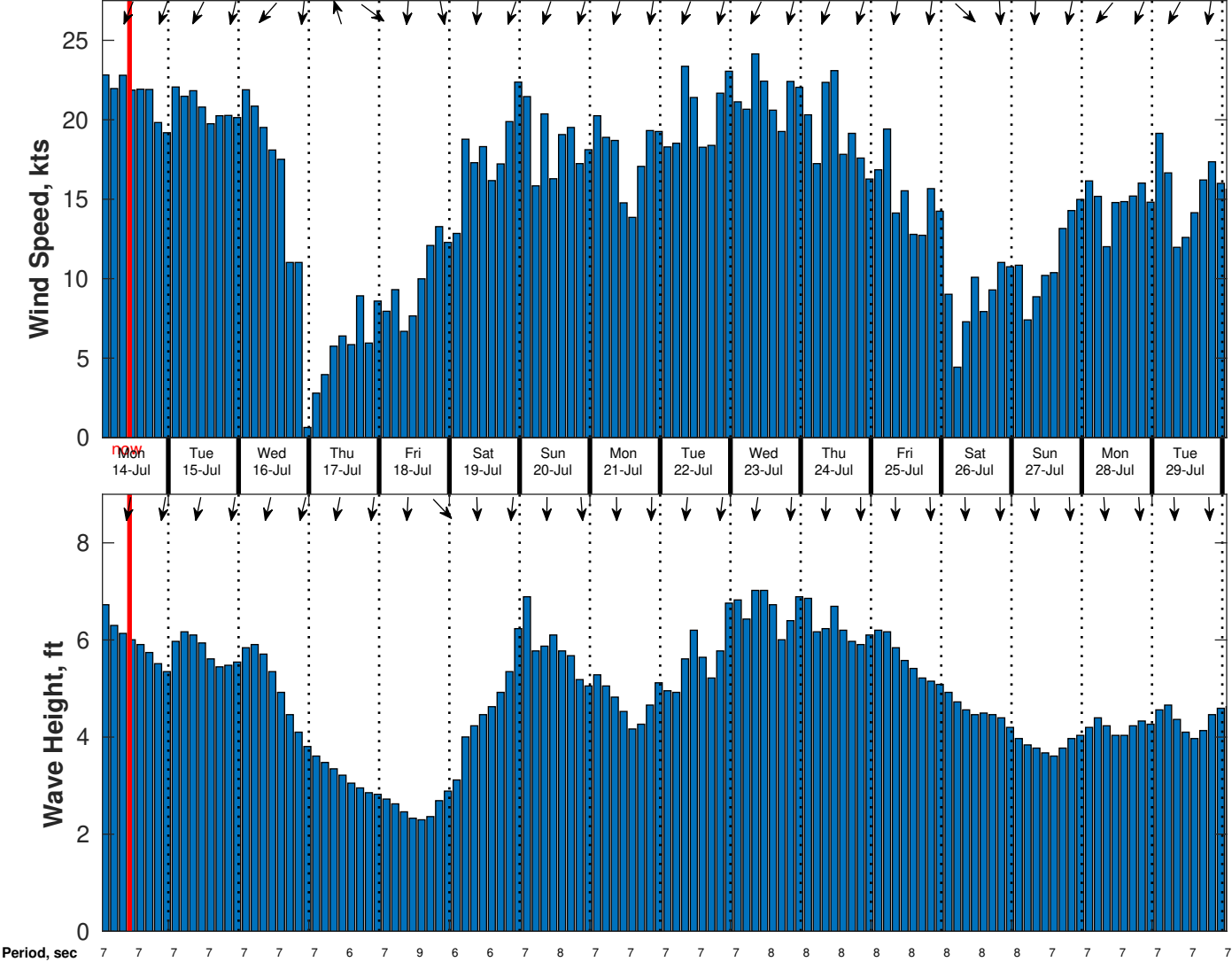
Wind & Wave Forecast for CSA (ONHYM) PPL EBS - Western Sahara from 13-Jul-2025 01:00:00 to 29-Jul-2025 01:00:00
