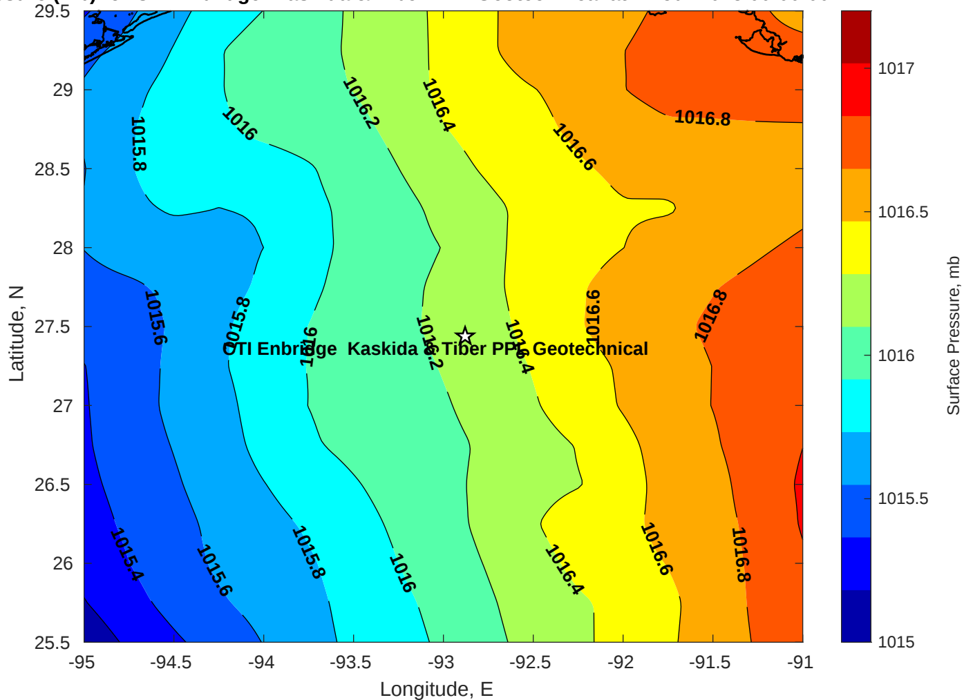
Surface Pressure (mb) for CTI Enbridge Kaskida & Tiber PPL Geotechnical at 14-Jul-2025 00:00:00
