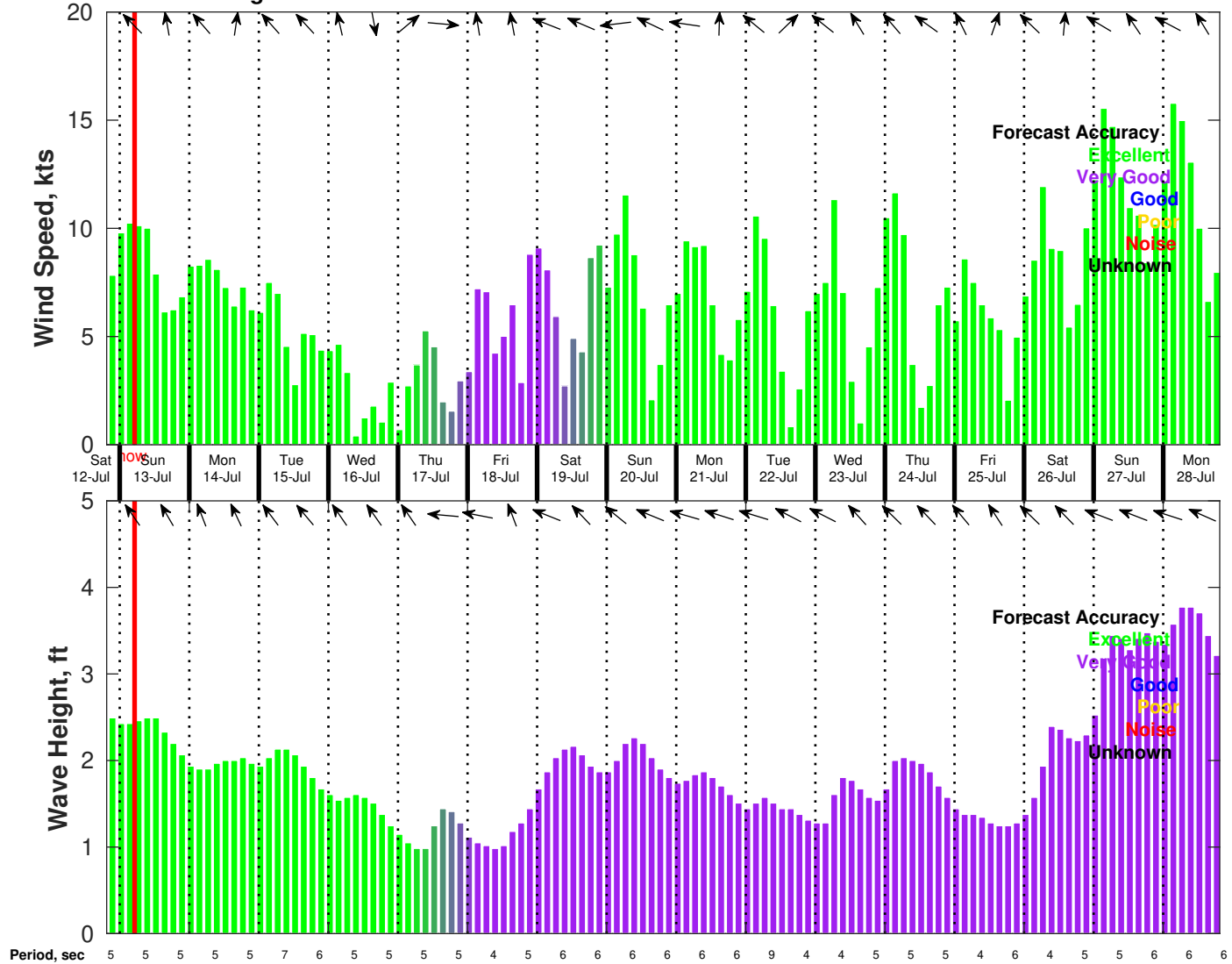
Wind & Wave Forecast for CTI Enbridge Kaskida & Tiber PPL Geotechnical from 12-Jul-2025 20:00:00 to 28-Jul-2025 20:00:00
