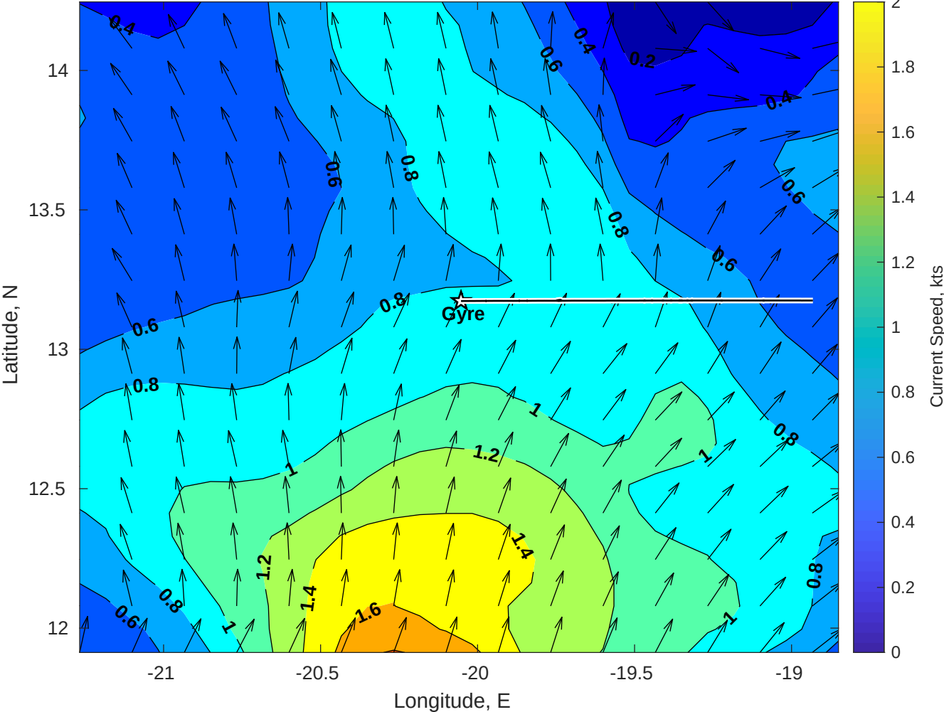
Surface Currents for Gyre at 12-Jul-2025 00:00:00
