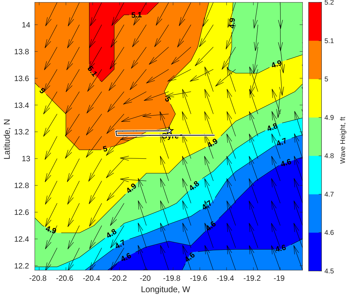
Wave Height (ft) for Gyre at 13-Jul-2025 09:00:00
