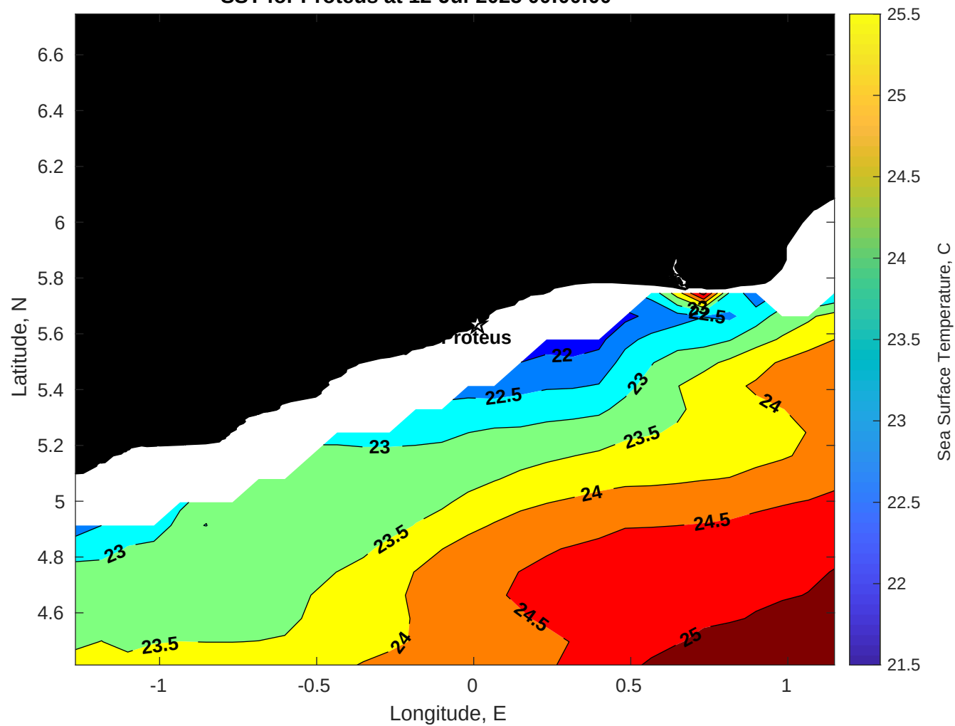
SST for Proteus at 12-Jul-2025 00:00:00
