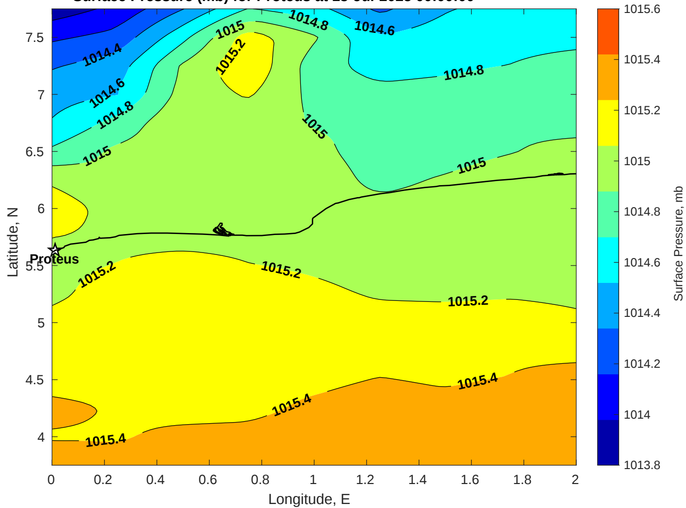
Surface Pressure (mb) for Proteus at 13-Jul-2025 00:00:00
