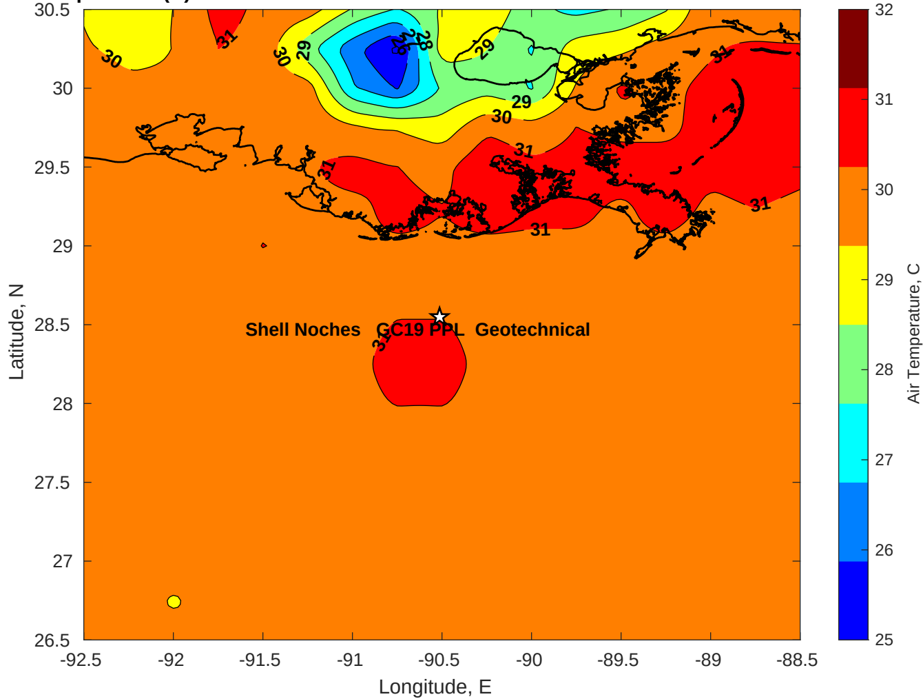
Air Temperature (C) for Shell Noches GC19 PPL Geotechnical at 13-Jul-2025
