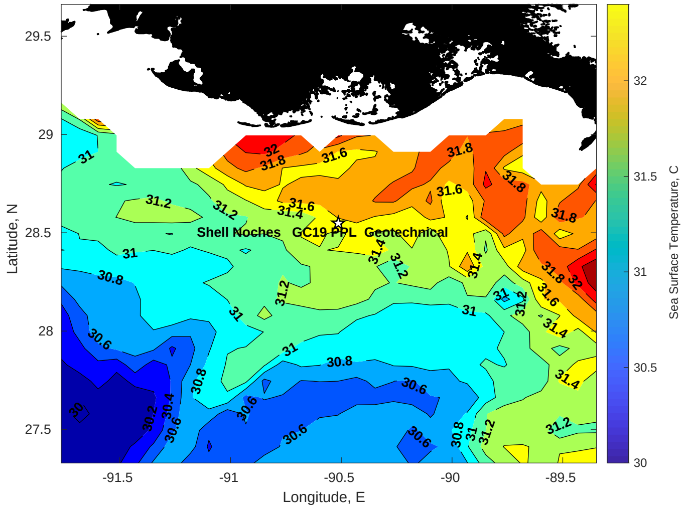
SST for Shell Noches GC19 PPL Geotechnical at 12-Jul-2025 00:00:00
