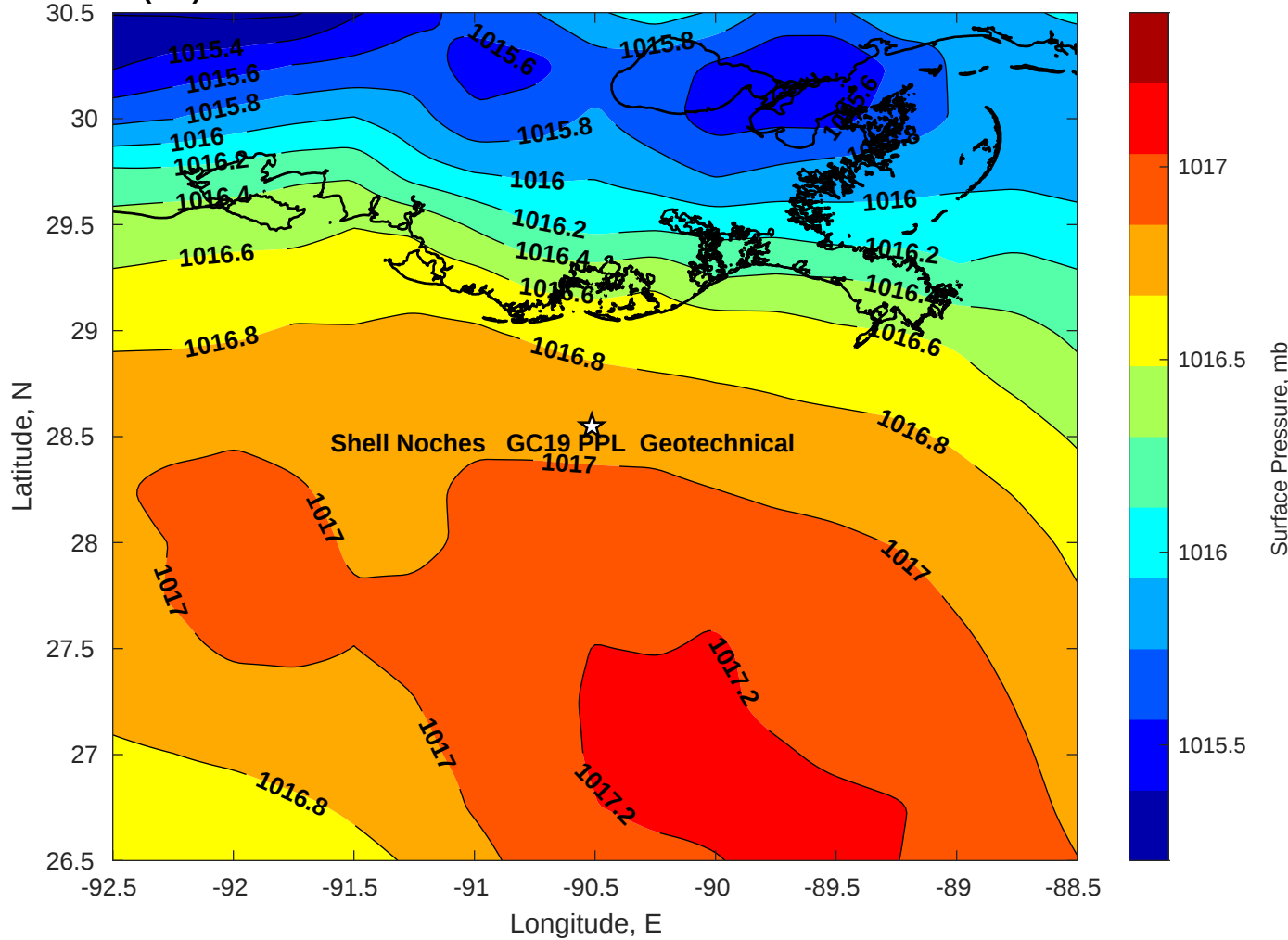
Surface Pressure (mb) for Shell Noches GC19 PPL Geotechnical at 15-Jul-2025 00:00:00
