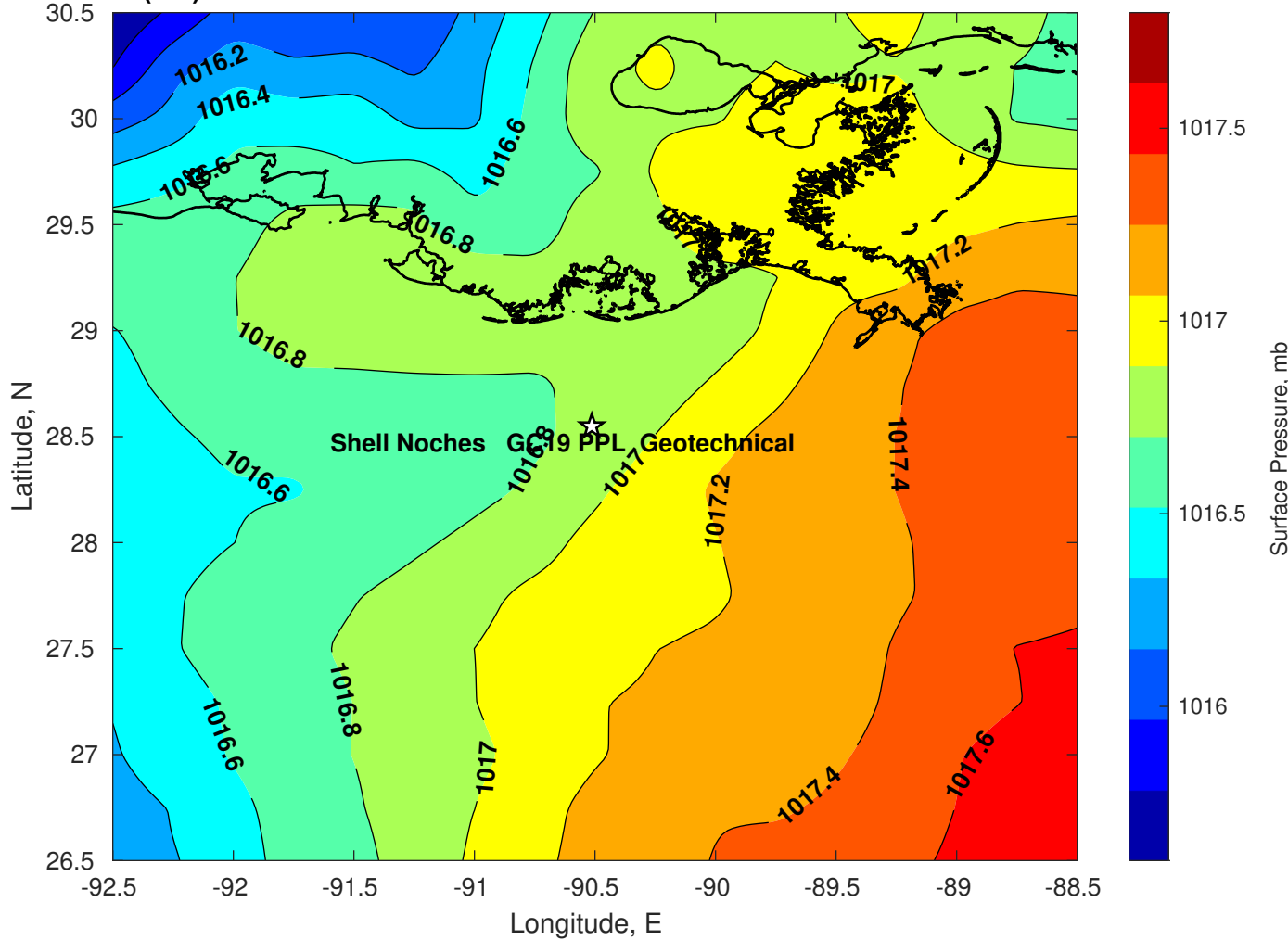
Surface Pressure (mb) for Shell Noches GC19 PPL Geotechnical at 14-Jul-2025 00:00:00
