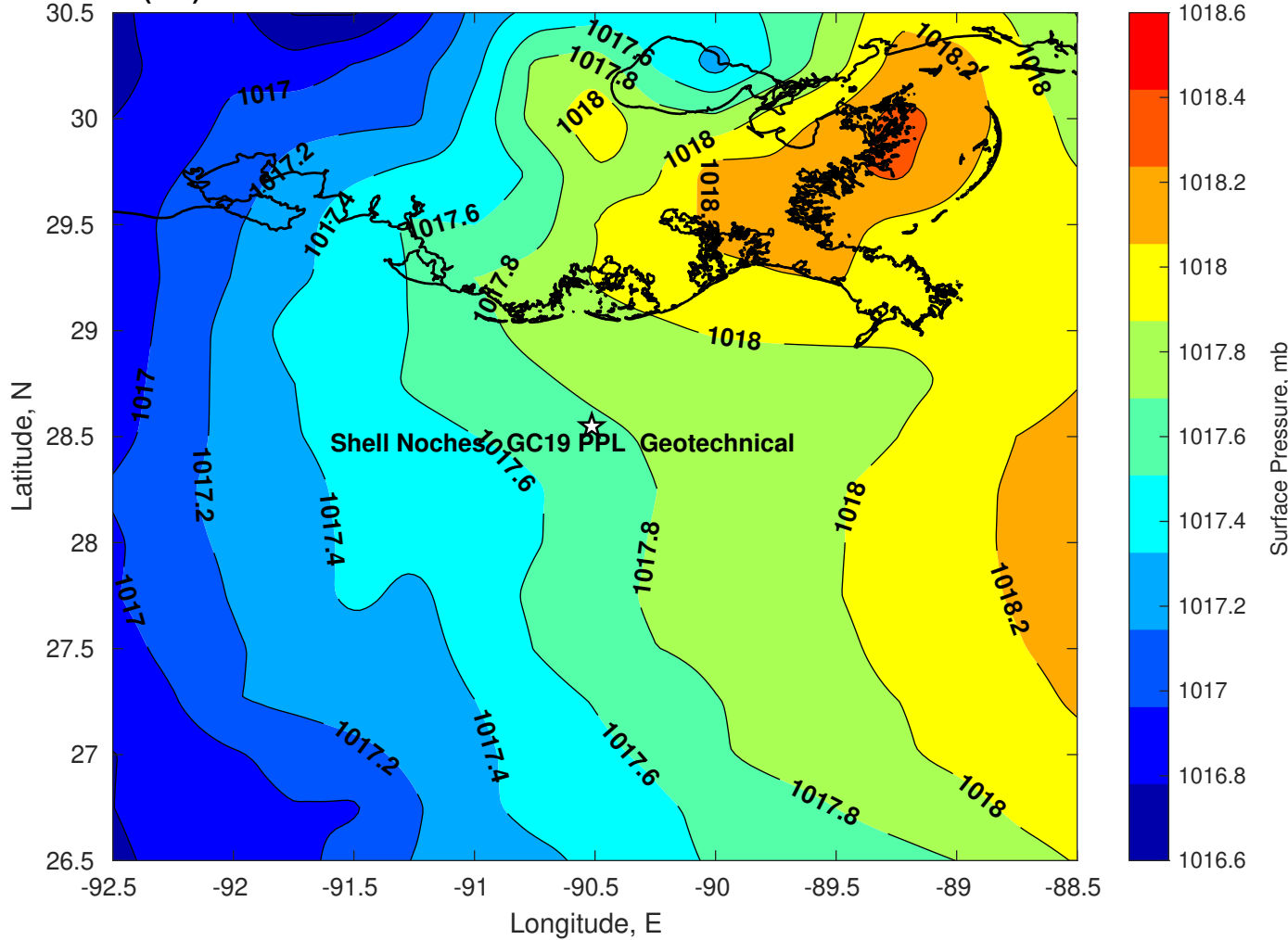
Surface Pressure (mb) for Shell Noches GC19 PPL Geotechnical at 13-Jul-2025 00:00:00
