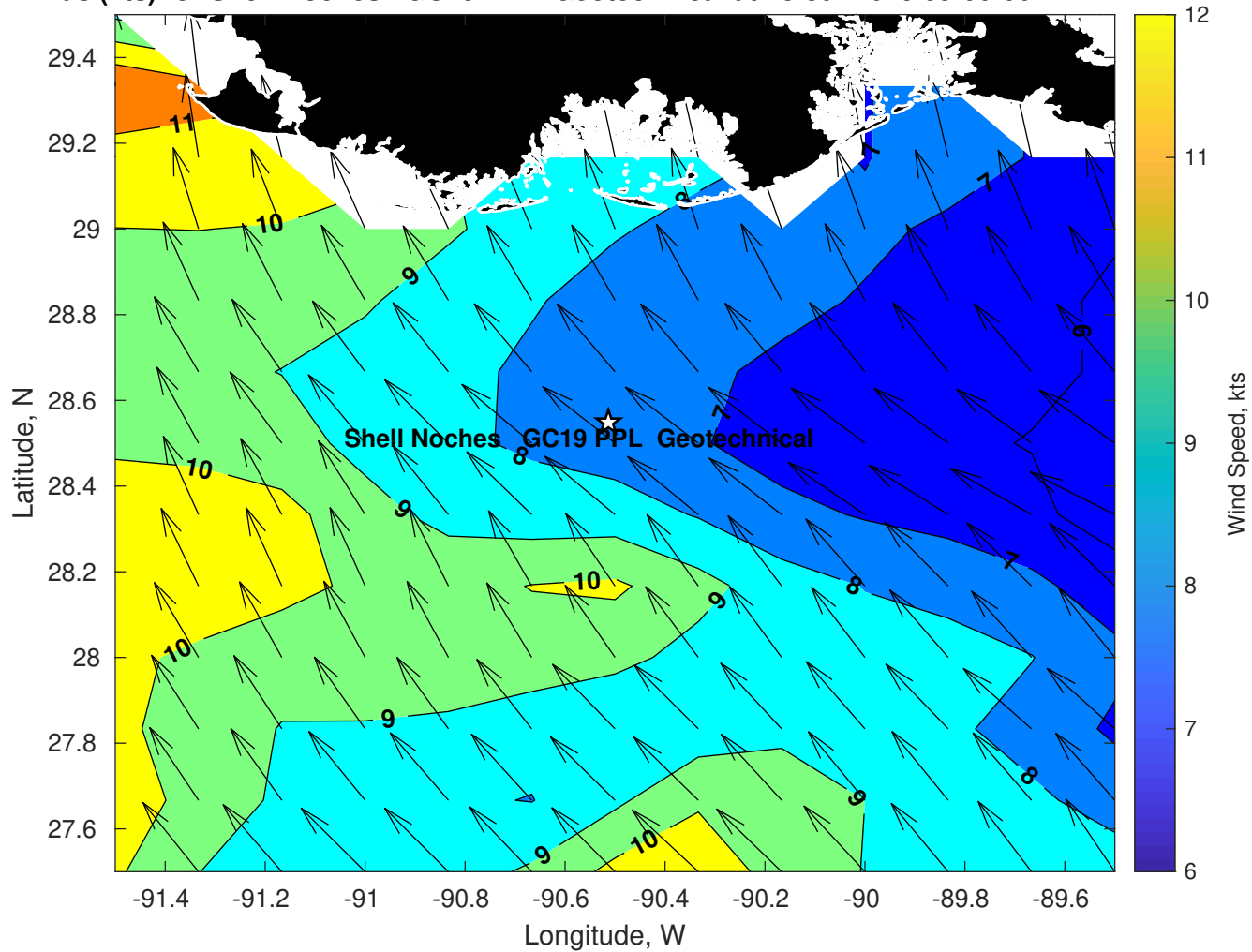
Winds (kts) for Shell Noches GC19 PPL Geotechnical at 13-Jul-2025 09:00:00
