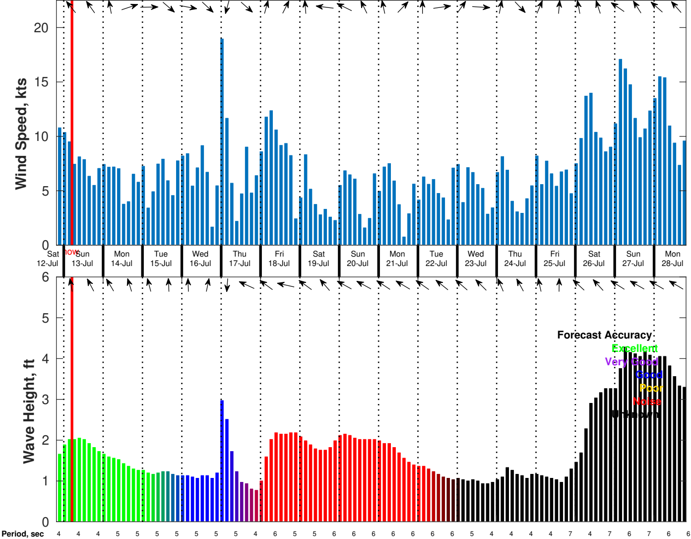
Wind & Wave Forecast for Shell Noches GC19 PPL Geotechnical from 12-Jul-2025 20:00:00 to 28-Jul-2025 20:00:00
