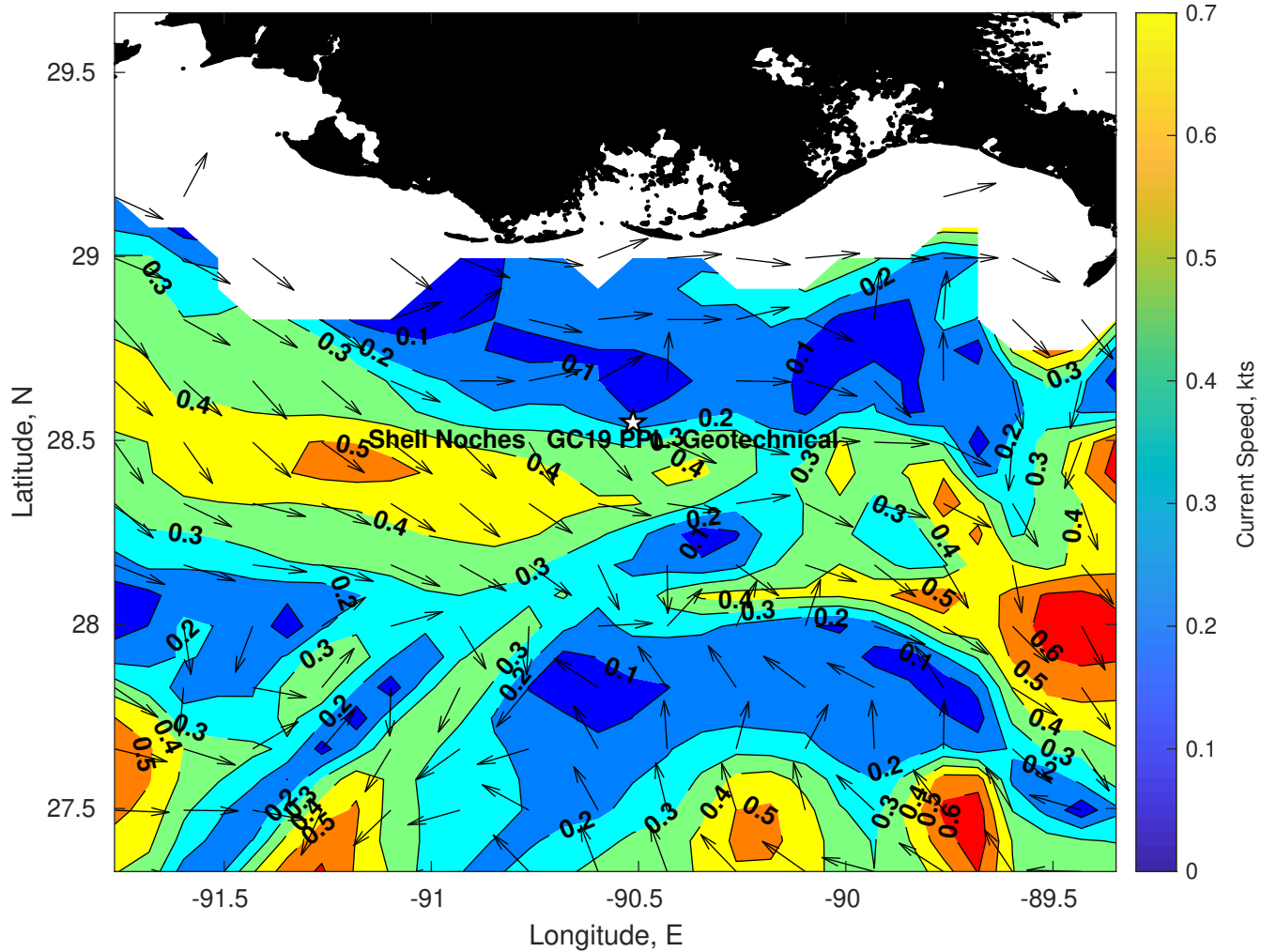
Surface Currents for Shell Noches GC19 PPL Geotechnical at 12-Jul-2025 00:00:00
