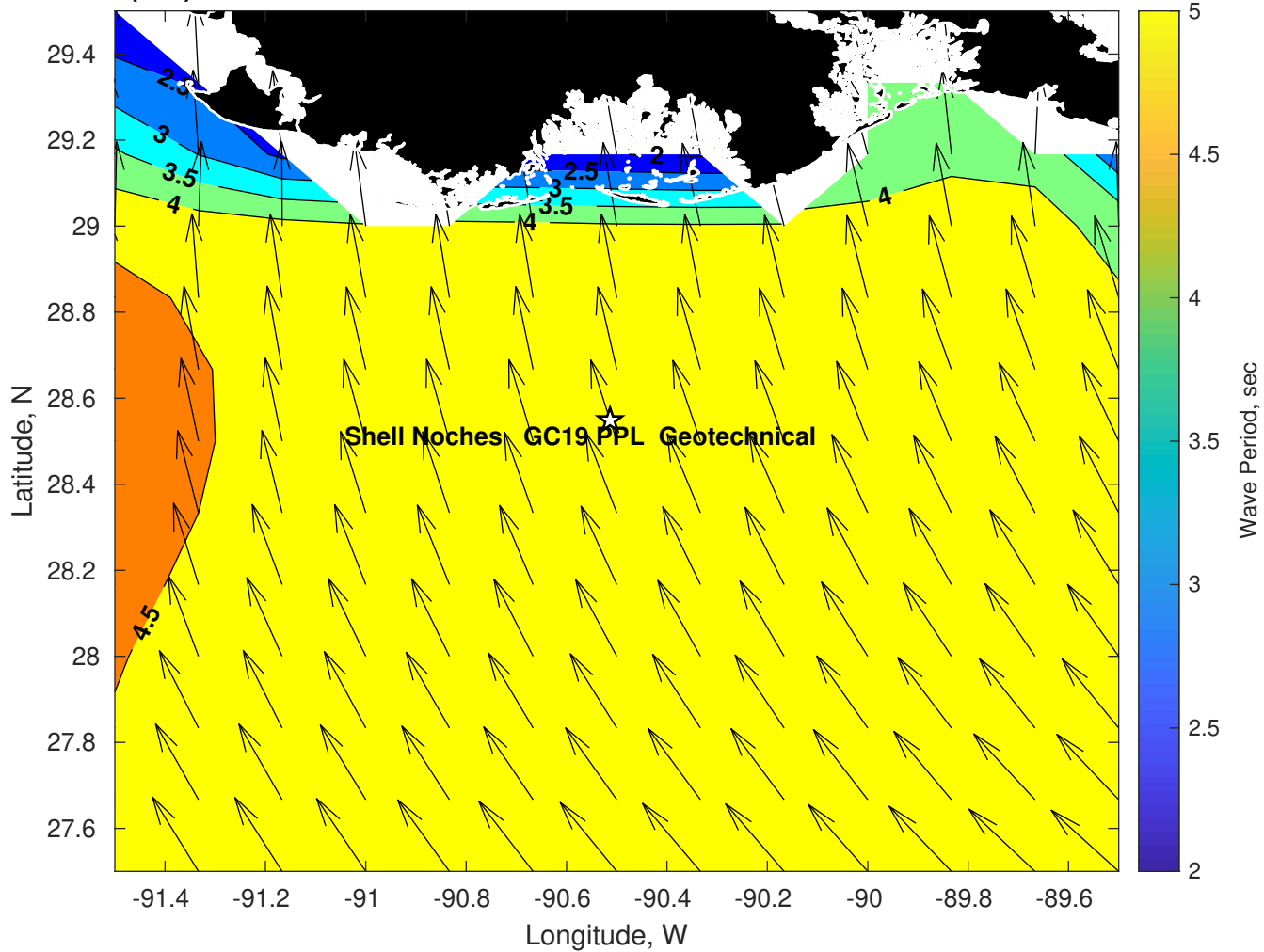
Wave Period (sec) for Shell Noches GC19 PPL Geotechnical at 13-Jul-2025 09:00:00
