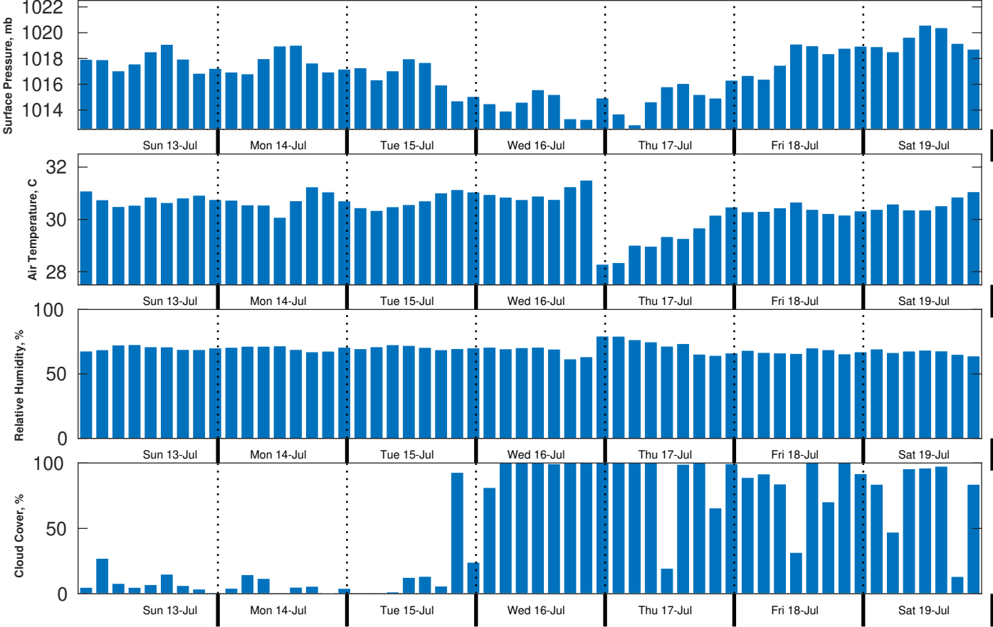
Met Forecast for Shell Noches GC19 PPL Geotechnical from 13-Jul-2025 00:00:00 to 20-Jul-2025 00:00:00
