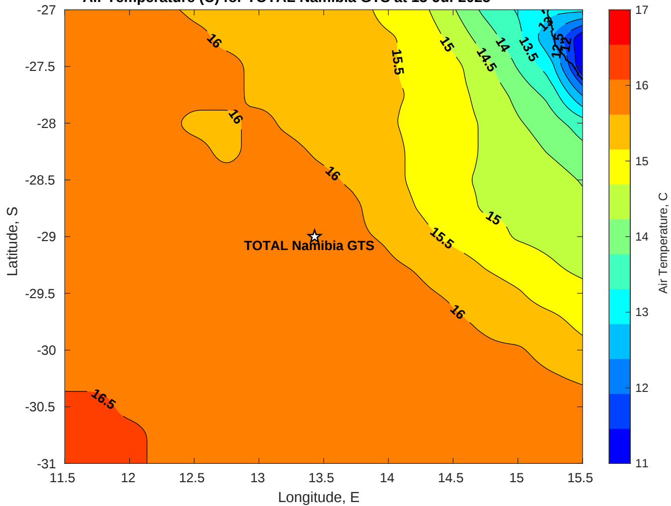
Air Temperature (C) for TOTAL Namibia GTS at 13-Jul-2025
