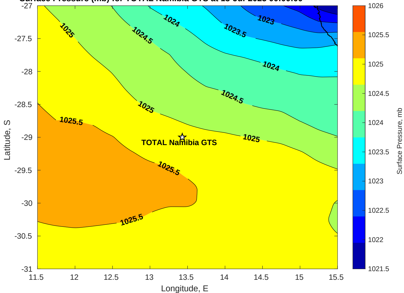
Surface Pressure (mb) for TOTAL Namibia GTS at 15-Jul-2025 00:00:00
