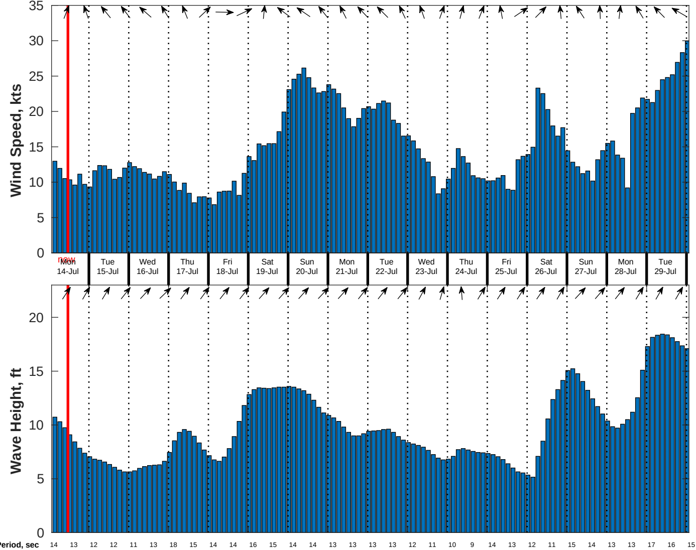
Wind & Wave Forecast for TOTAL Namibia GTS from 13-Jul-2025 02:00:00 to 29-Jul-2025 02:00:00
