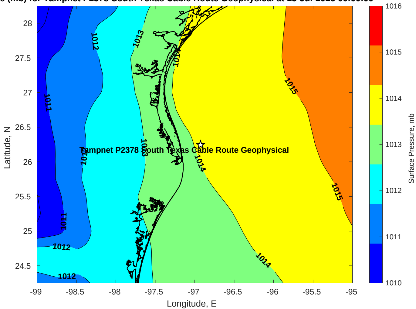
Pressure (mb) for Tampnet P2378 South Texas Cable Route Geophysical at 13-Jul-2025 00:00:00
