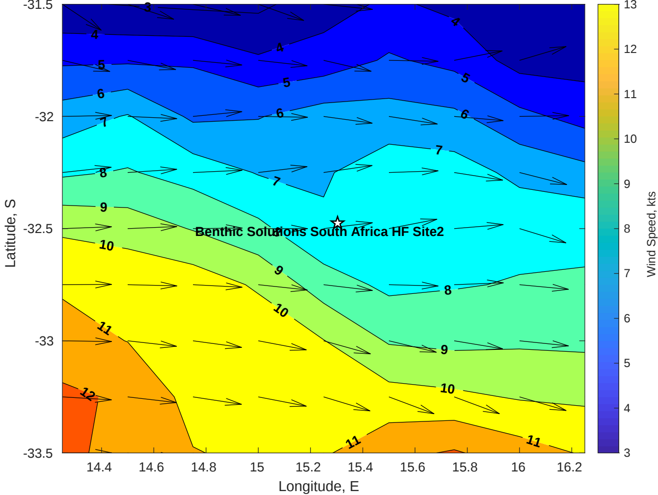
Winds (kts) for Benthic Solutions South Africa HF Site2 at 13-Jul-2025 21:00:00
