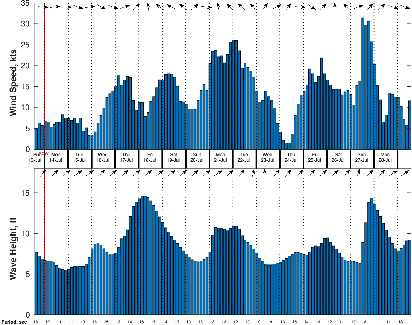
Wind & Wave Forecast for Benthic Solutions South Africa HF Site3 from 13-Jul-2025 14:00:00 to 29-Jul-2025 14:00:00
