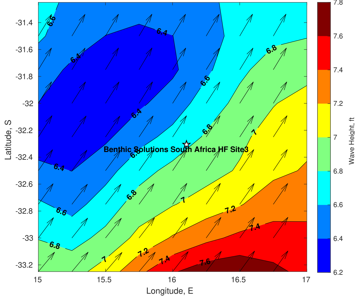
Wave Height (ft) for Benthic Solutions South Africa HF Site3 at 13-Jul-2025 21:00:00
