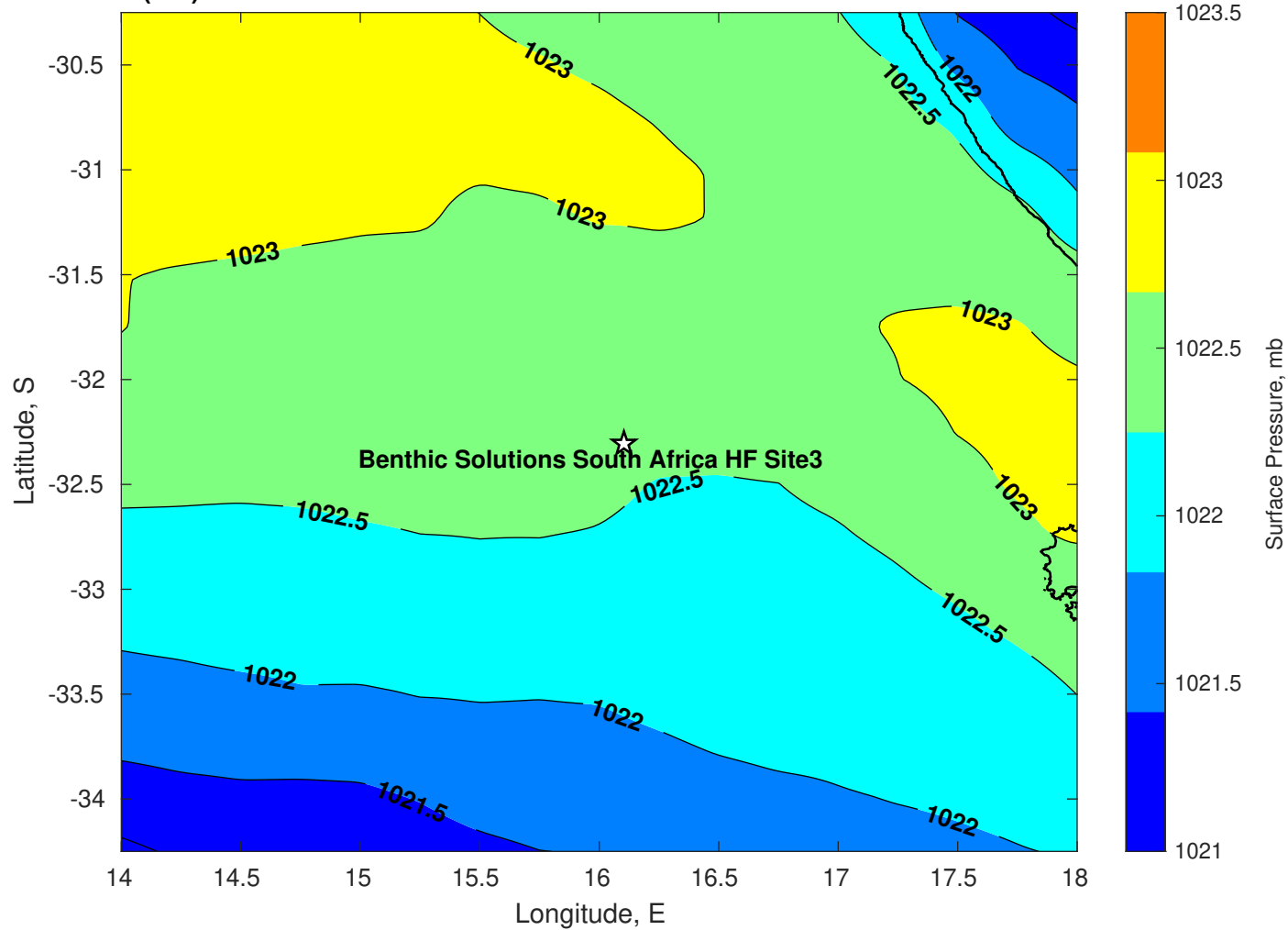
Surface Pressure (mb) for Benthic Solutions South Africa HF Site3 at 15-Jul-2025 12:00:00
