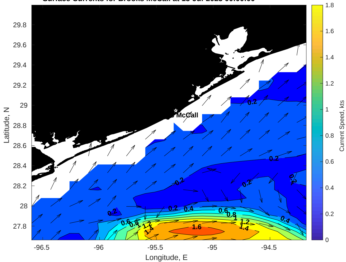
Surface Currents for Brooks McCall at 13-Jul-2025 00:00:00
