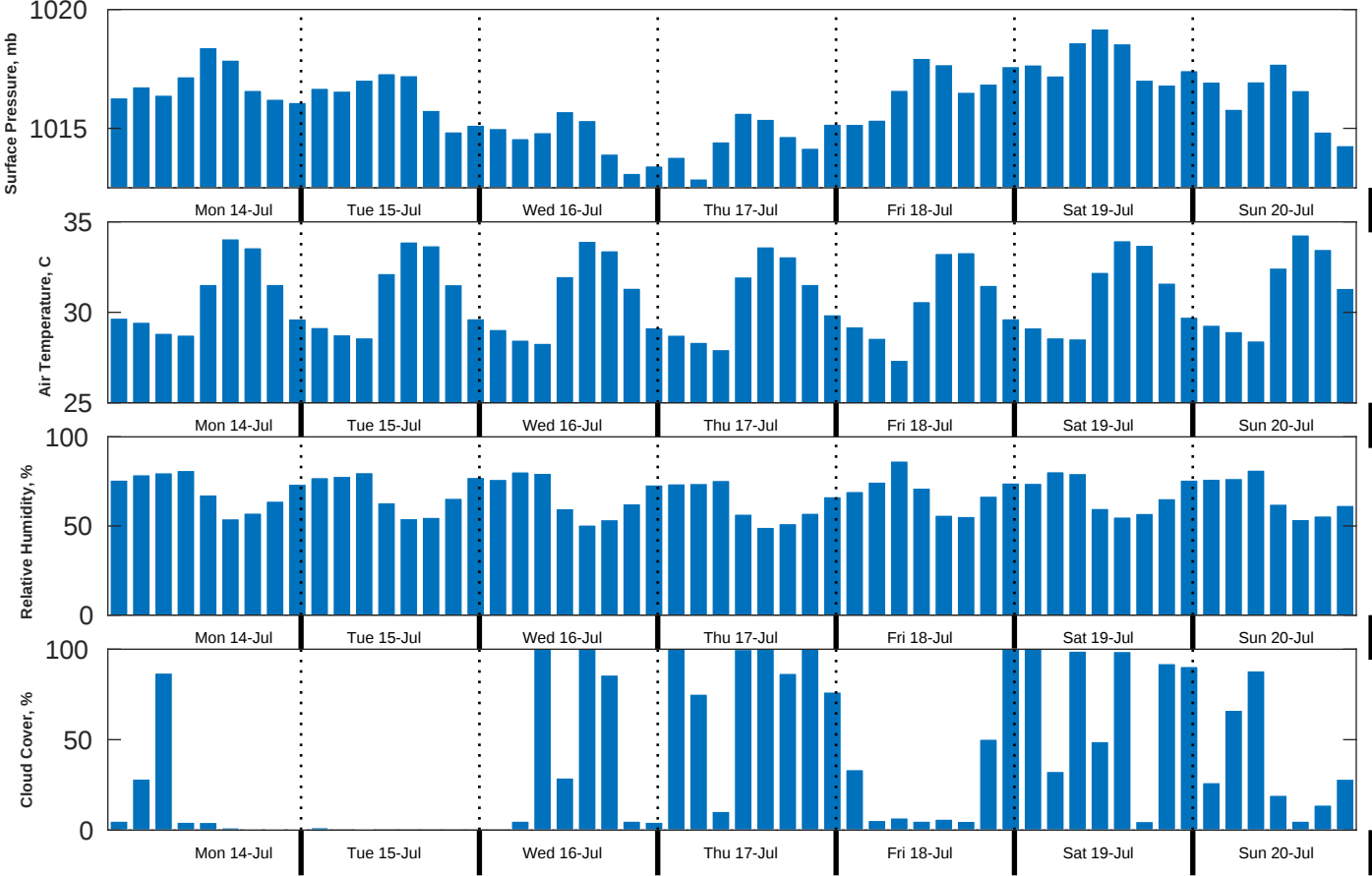
Met Forecast for Brooks McCall from 14-Jul-2025 00:00:00 to 21-Jul-2025 00:00:00
