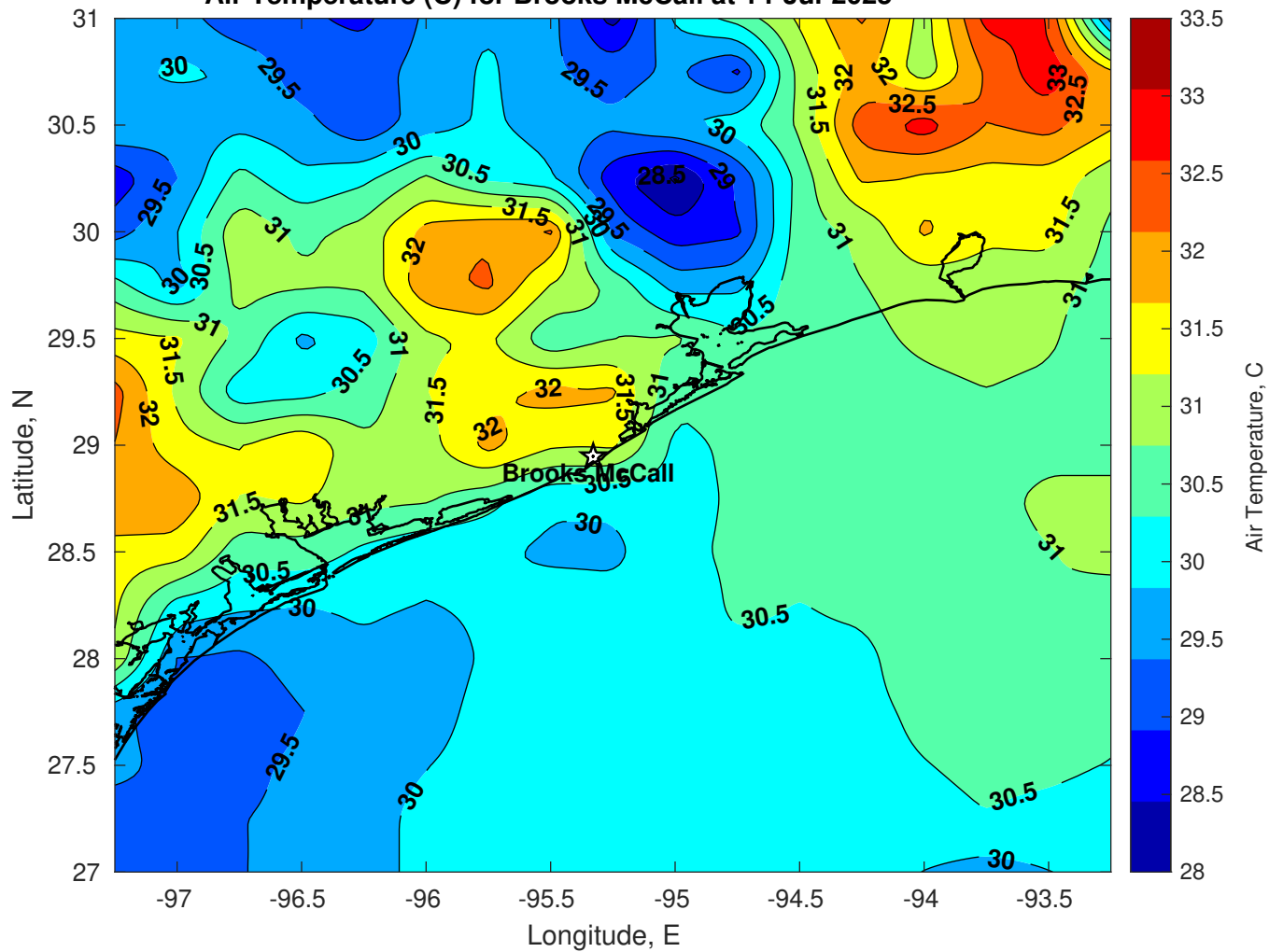
Air Temperature (C) for Brooks McCall at 14-Jul-2025
