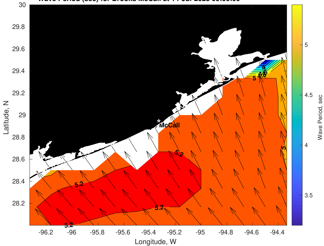
Wave Period (sec) for Brooks McCall at 14-Jul-2025 09:00:00
