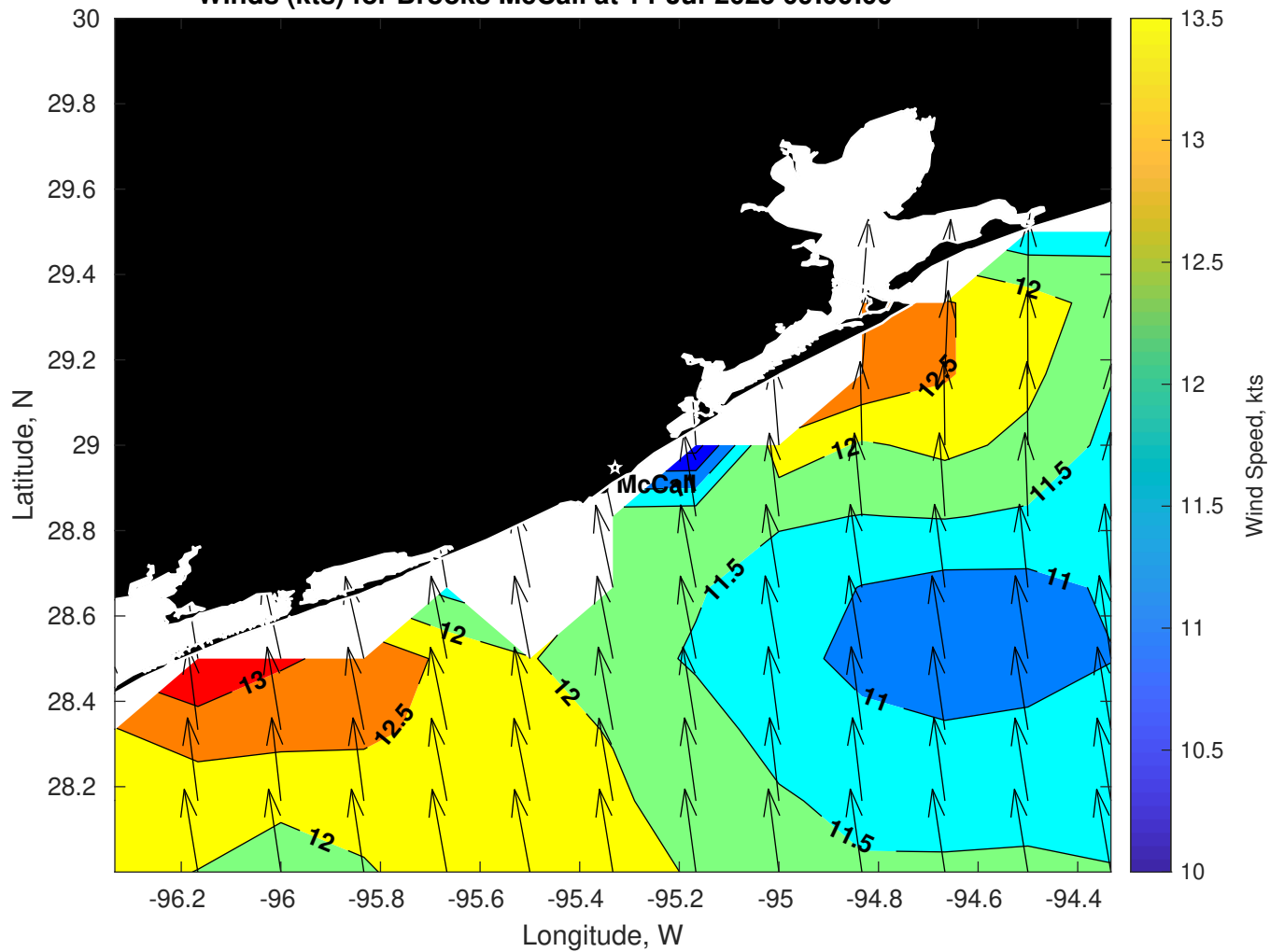
Winds (kts) for Brooks McCall at 14-Jul-2025 09:00:00
