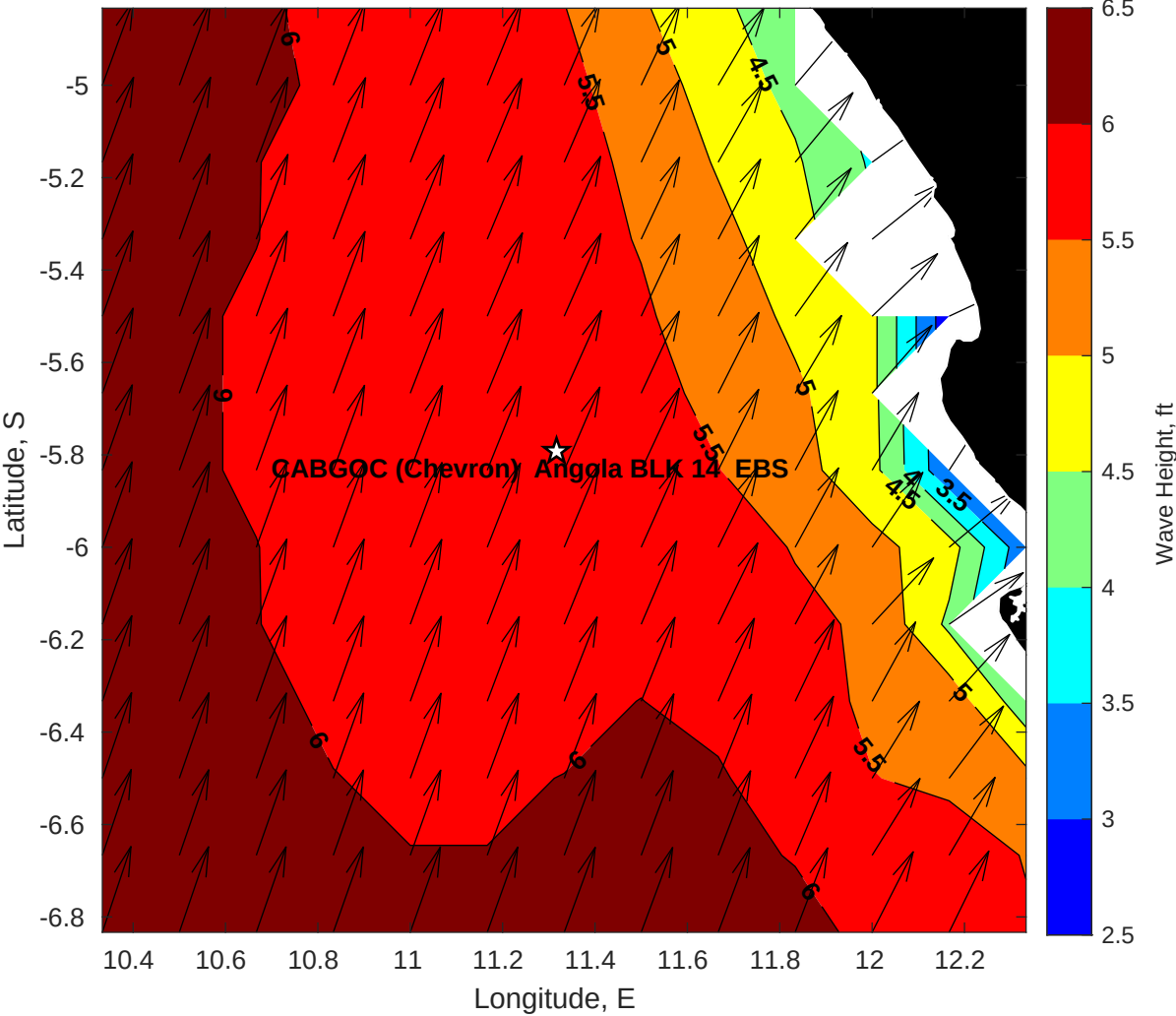
Wave Height (ft) for CABGOC (Chevron) Angola BLK 14 EBS at 13-Jul-2025 21:00:00
