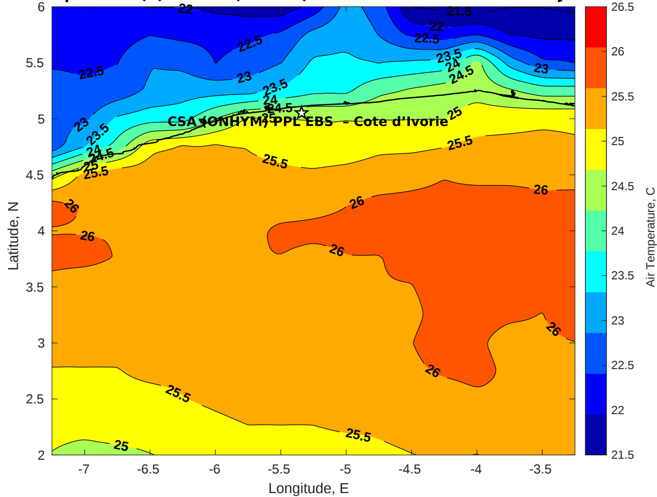
Air Temperature (C) for CSA (ONHYM) PPL EBS - Cote d'Ivoire at 14-Jul-2025
