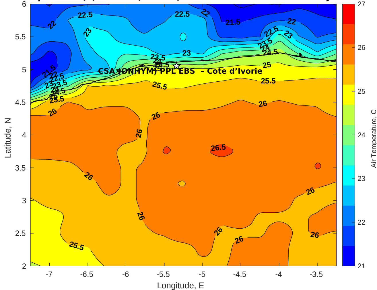
Air Temperature (C) for CSA (ONHYM) PPL EBS - Cote d'Ivoire at 14-Jul-2025
