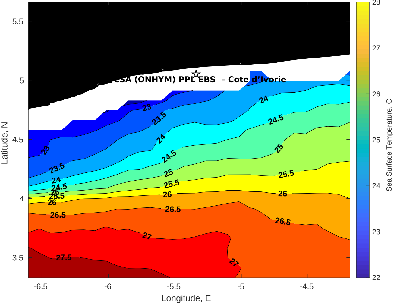
SST for CSA (ONHYM) PPL EBS - Cote d'Ivoire at 13-Jul-2025 00:00:00
